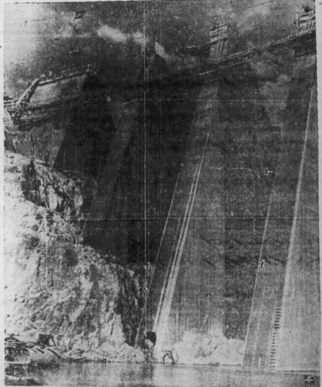
ROCKY IS THE ROAD these Bartlett dam buttresses must climb, reaching an upper level of the 270-foot multiple-arch dam being built on the Verde river in Arizona. This is the right abutment. The dam, which is four-fifths complete, comprises arches built at an angle and supported by these buttresses. The dam will create a reservoir of 200,000 acre feet capacity to serve the additional irrigation needs of the highly developed Salt river federal reclamation project.
