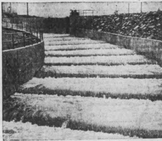
SO THE U. S. government provided ladders like this one so the salmon could get around the dam. Each step of the ladder is one foot high.
