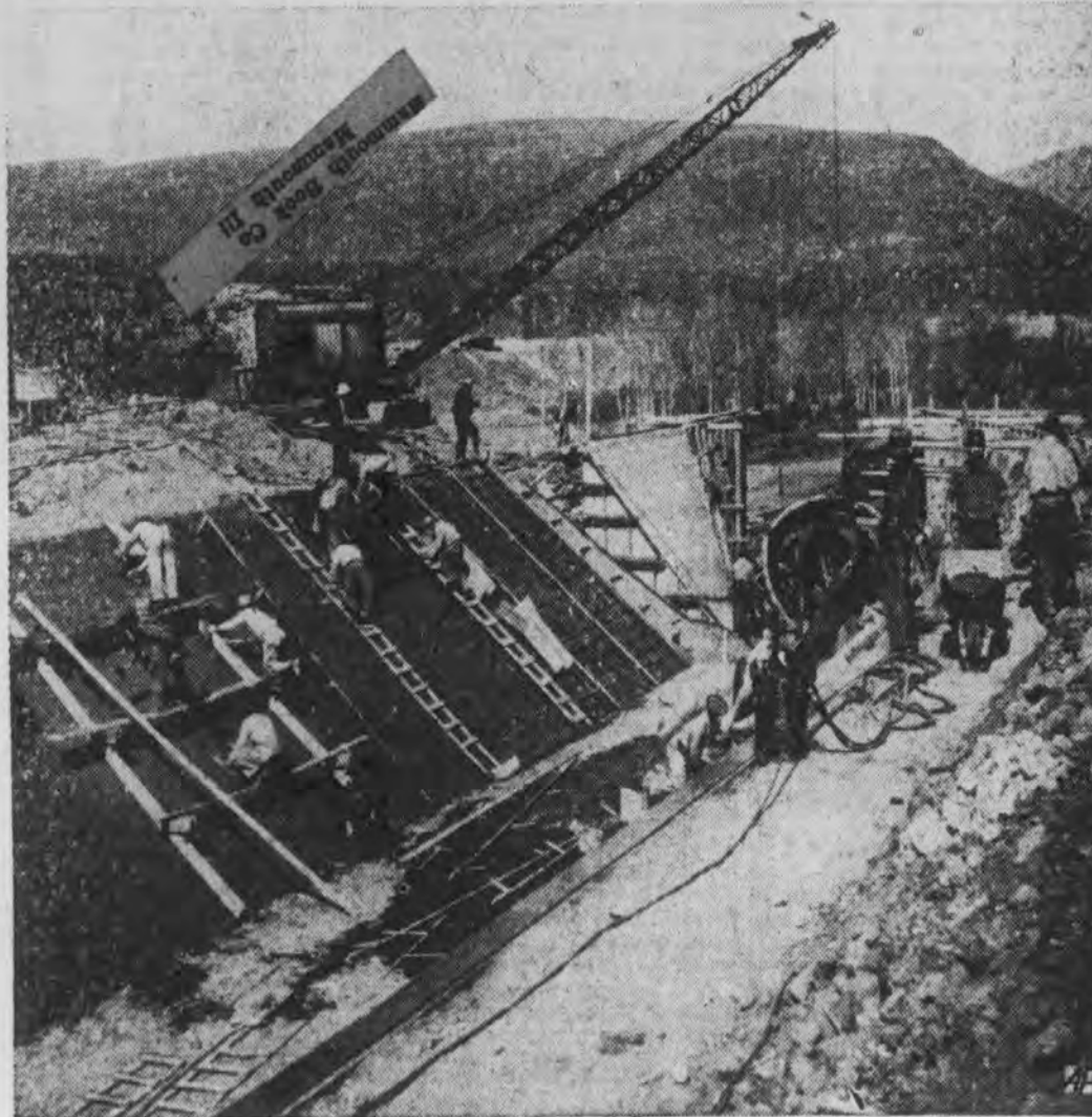
The Federal Bureau of Reclamation pushes work on Washington State canals which will serve Rosa division, a 72,000-acre addition to the Yakima irrigation project. Above are canal-fining operations on Pomona siphon, eight miles above Coulee dam, is about half done.
