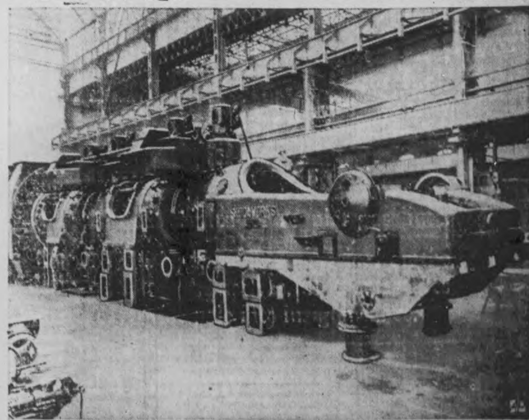
MUNITIONS—NOT MALT shoves beer-brewing Pilsen into the news, since war threats have put Skoda munitions plant with its machines like this on a 24-hour basis. The Skoda works employs more than 38,000 workers in Czechoslovakia alone; there are Skoda branch plants in Rumania and Poland.
