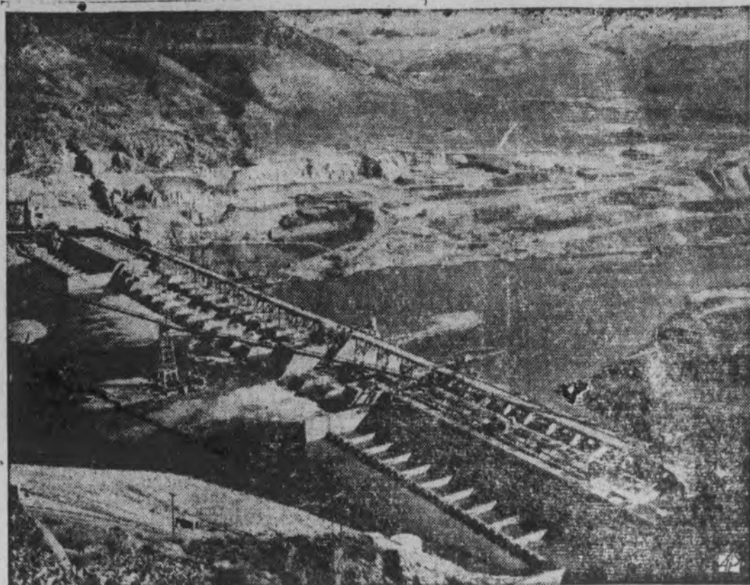
HALF-WAY MARK IS REACHED on Grand Coulee dam, $114,000,000 federal project on Columbia river, Washington. Dam will be 550 feet high, contain 11,250,000 cubic yards of concrete.
