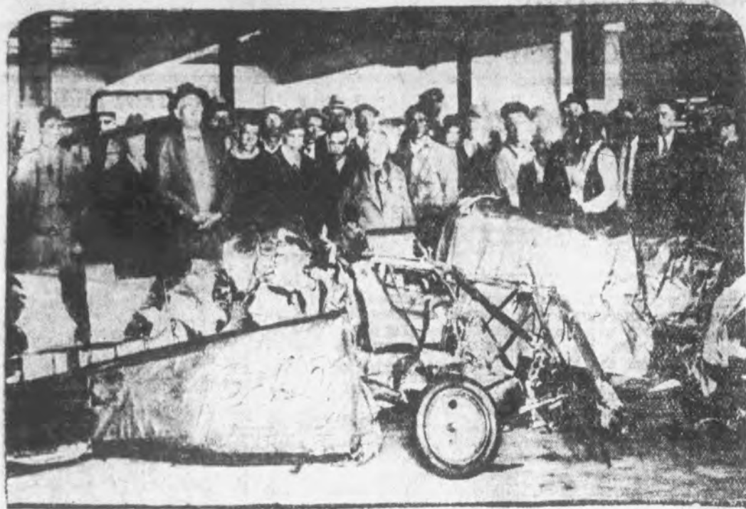
Here is all that is left of the Ford baby plane, piloted by Harry Brooks, the wreckage having been washed ashore near Melbourne, Fla. The tiny plane in which the pilot completed a hop from Michigan to Florida, dived into the sea several days ago, and it is now believed certain that Brooks was drowned.
