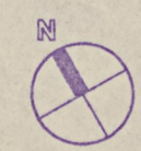
F1401 THIRD FLOOR FURNITURE PLAN SCALE: 1/8"=1'-0" (2,1754-3) (RSP/RSD) (2,1754-2) (RAC/RAD)
