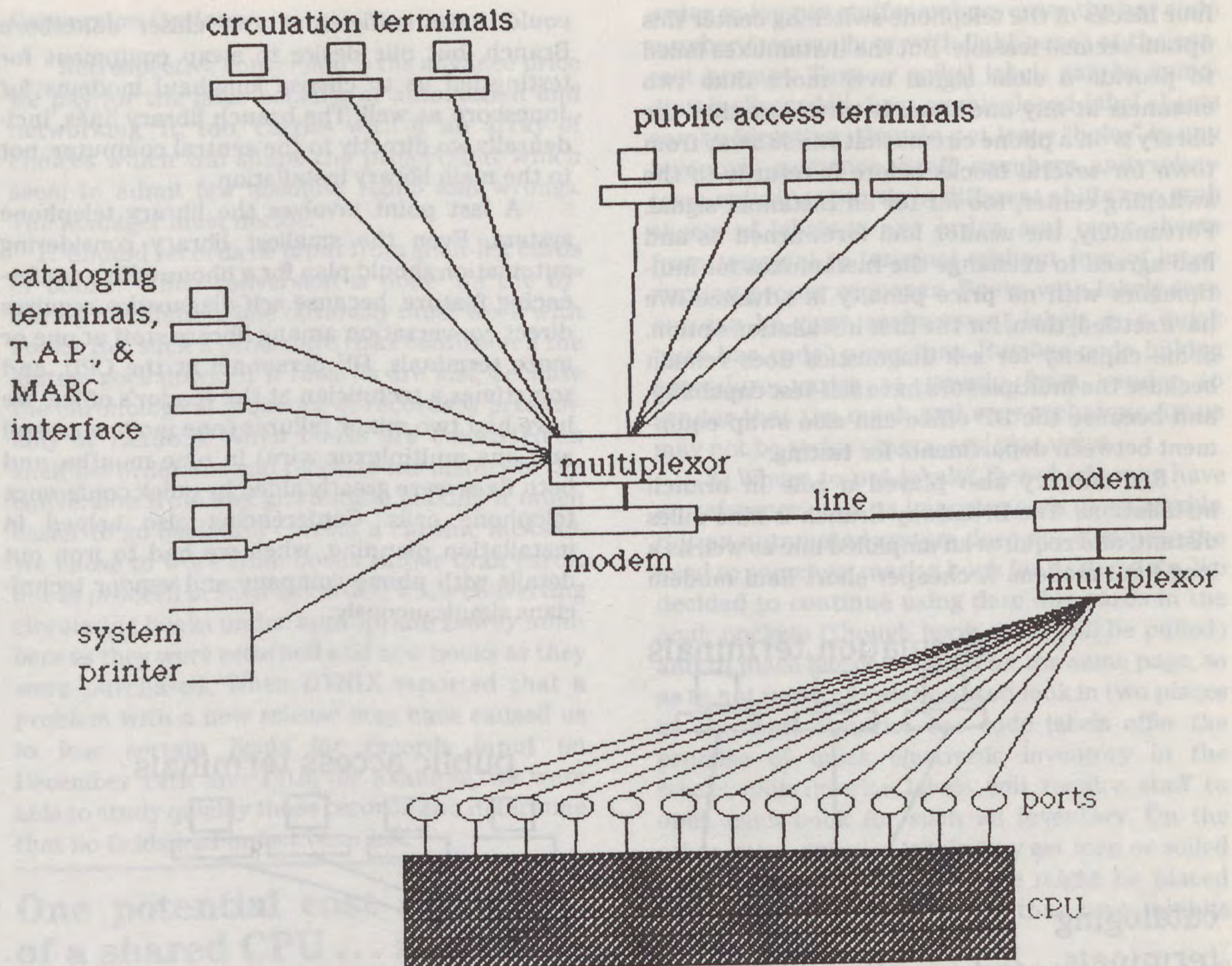
Figure III. Lee County Library's hardware installation layout.
