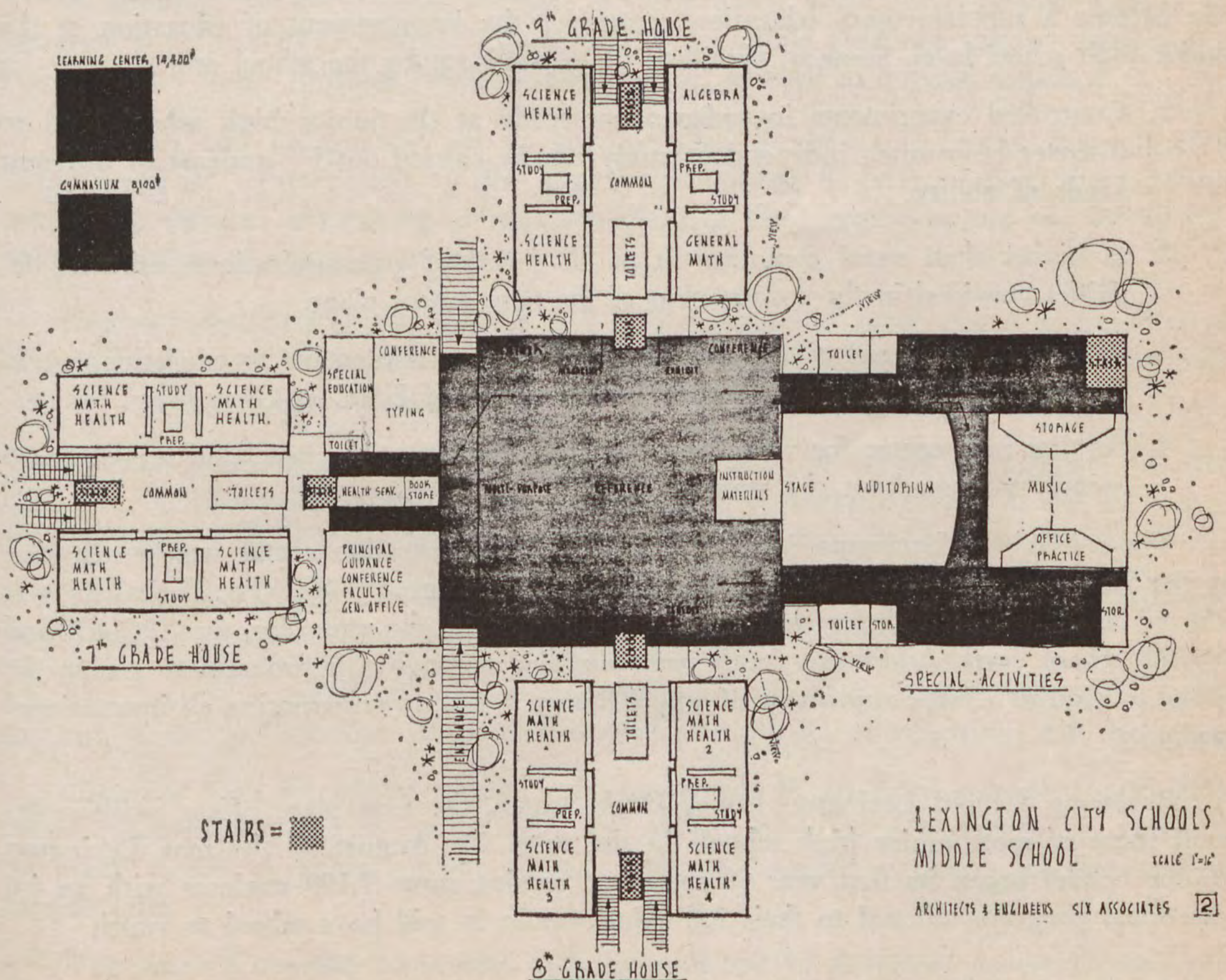
MAIN FLOOR, LEXINGTON MIDDLE SCHOOL — SCALE: 1"=16'
