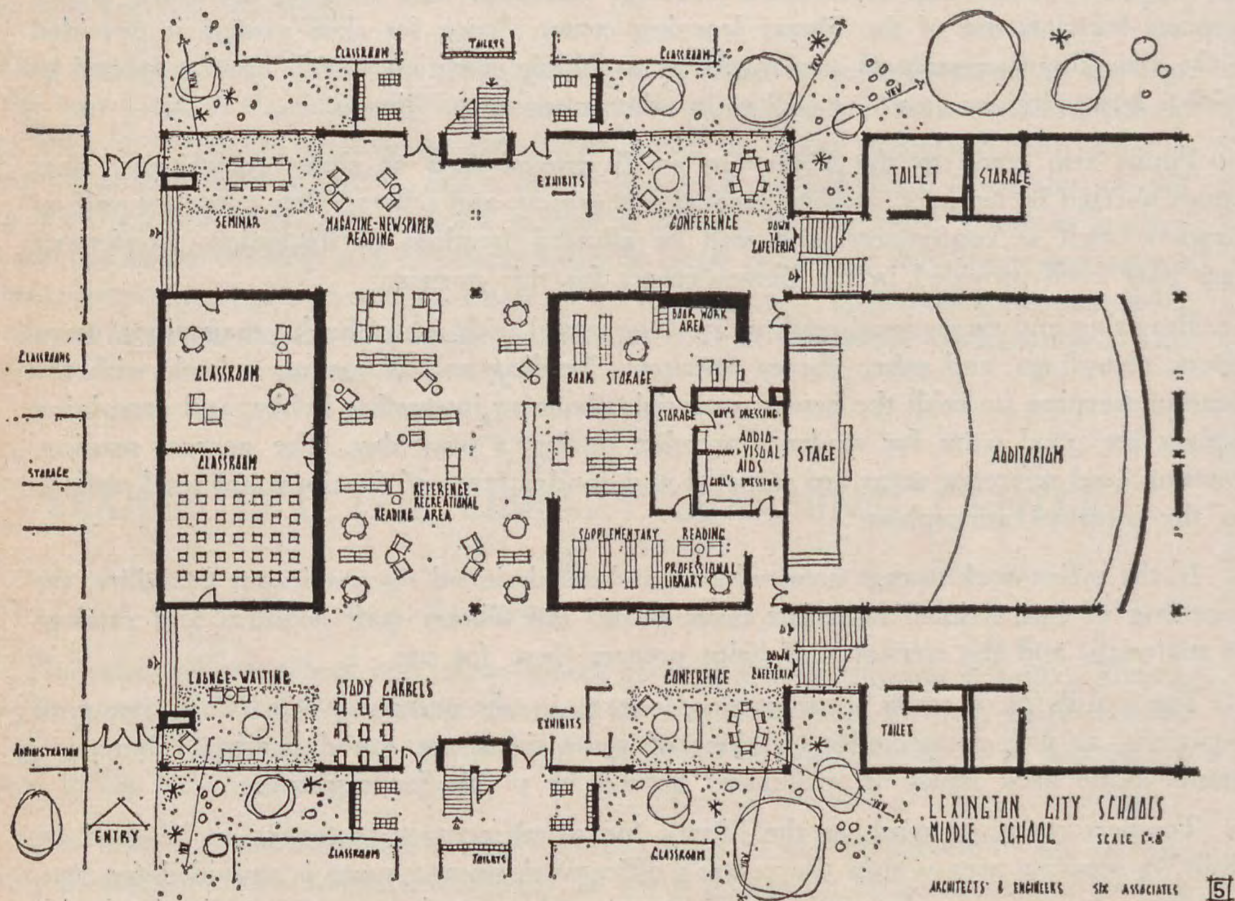
LIBRARY LEARNING CENTER — LEXINGTON MIDDLE SCHOOL — SCALE: 1"=8'
