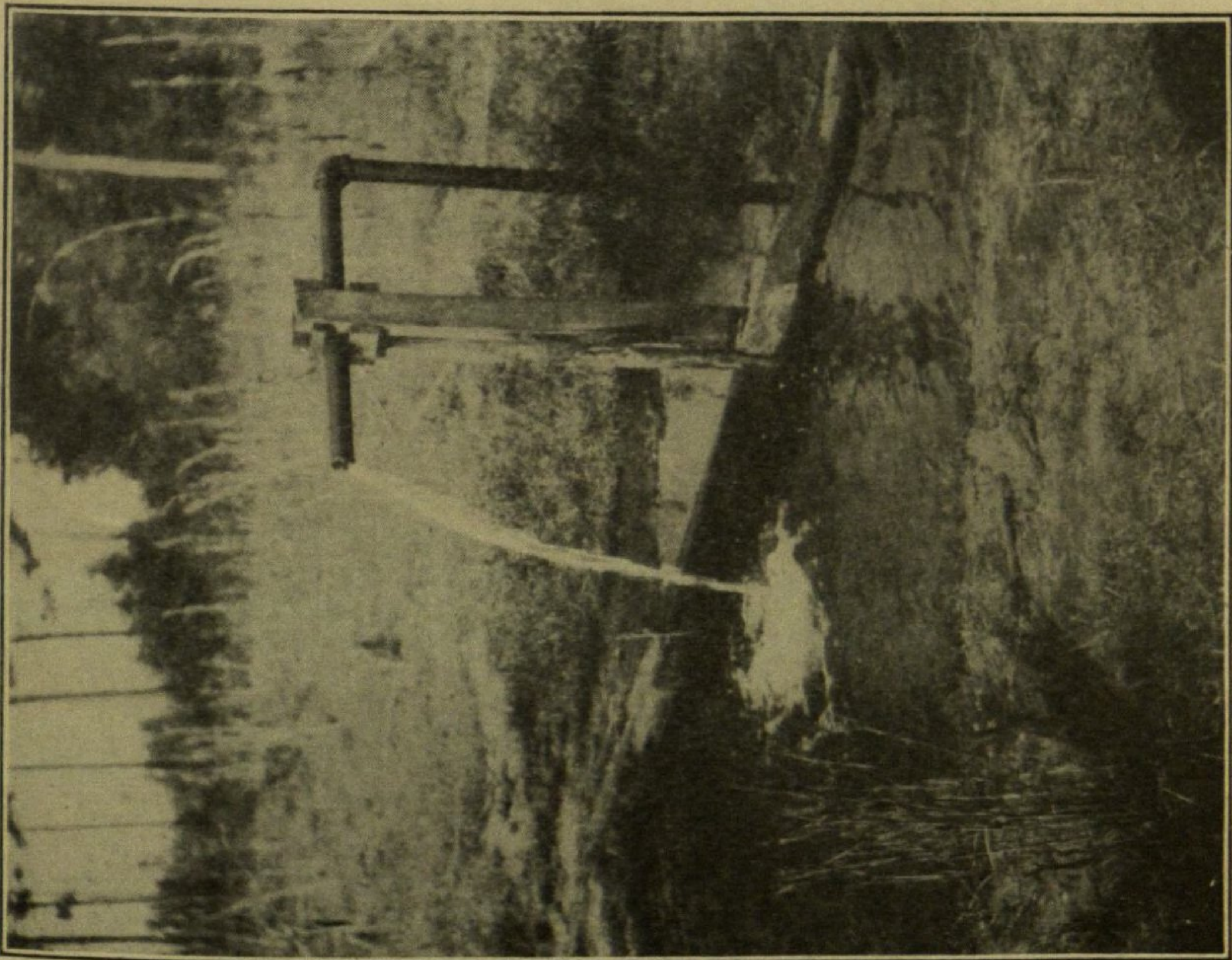
A.—Flowing well from strata of the Black Creek formation at fair grounds, Lumberton, N. C.
