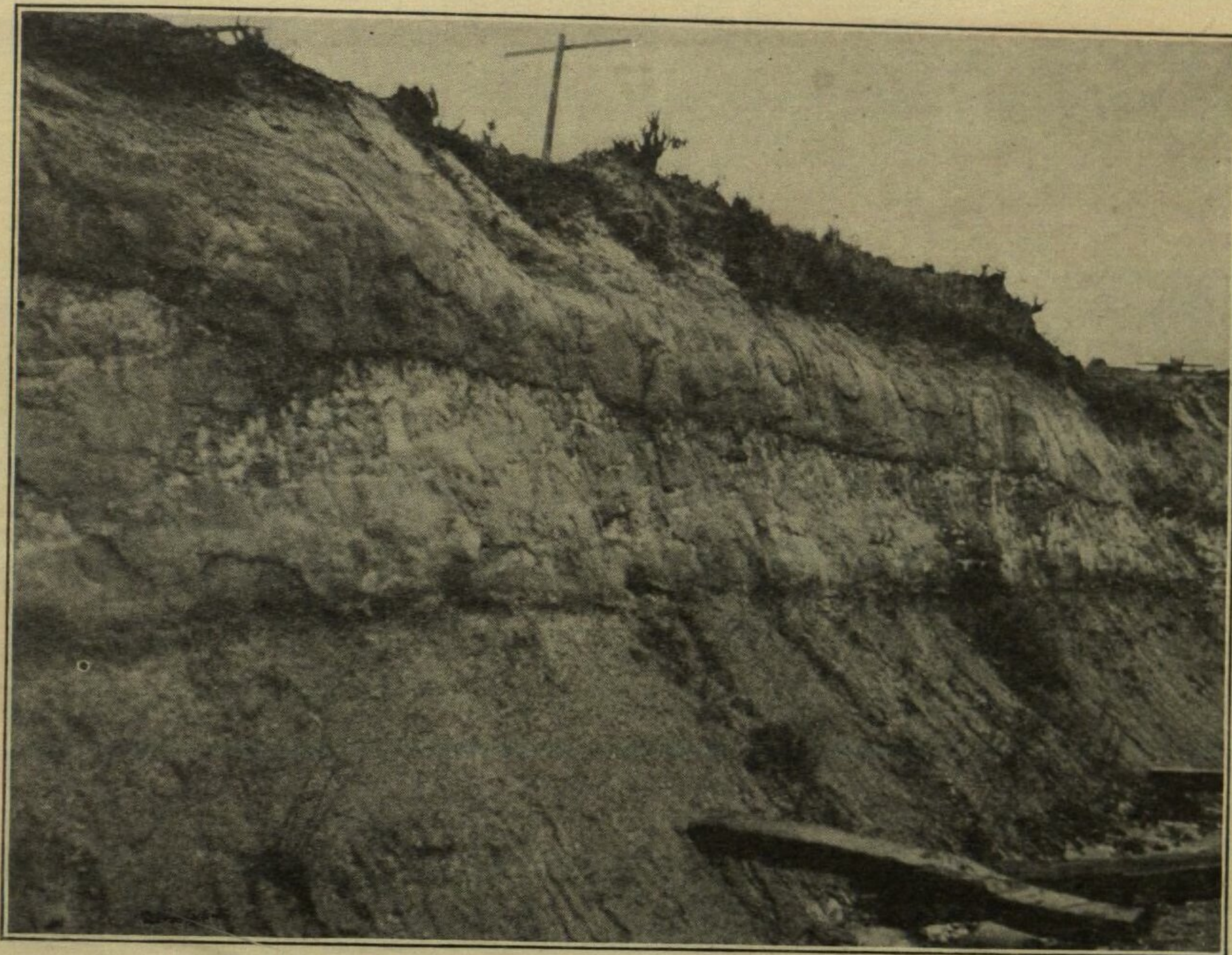
A.—Exposure of the Coharie formation resting unconformably upon the Patuxent formation; cut of the Atlantic Coast Line Railroad, 2\frac{3}{4} miles northeast of Four Oaks, near Corinth Church, Johnston County, N. C.
