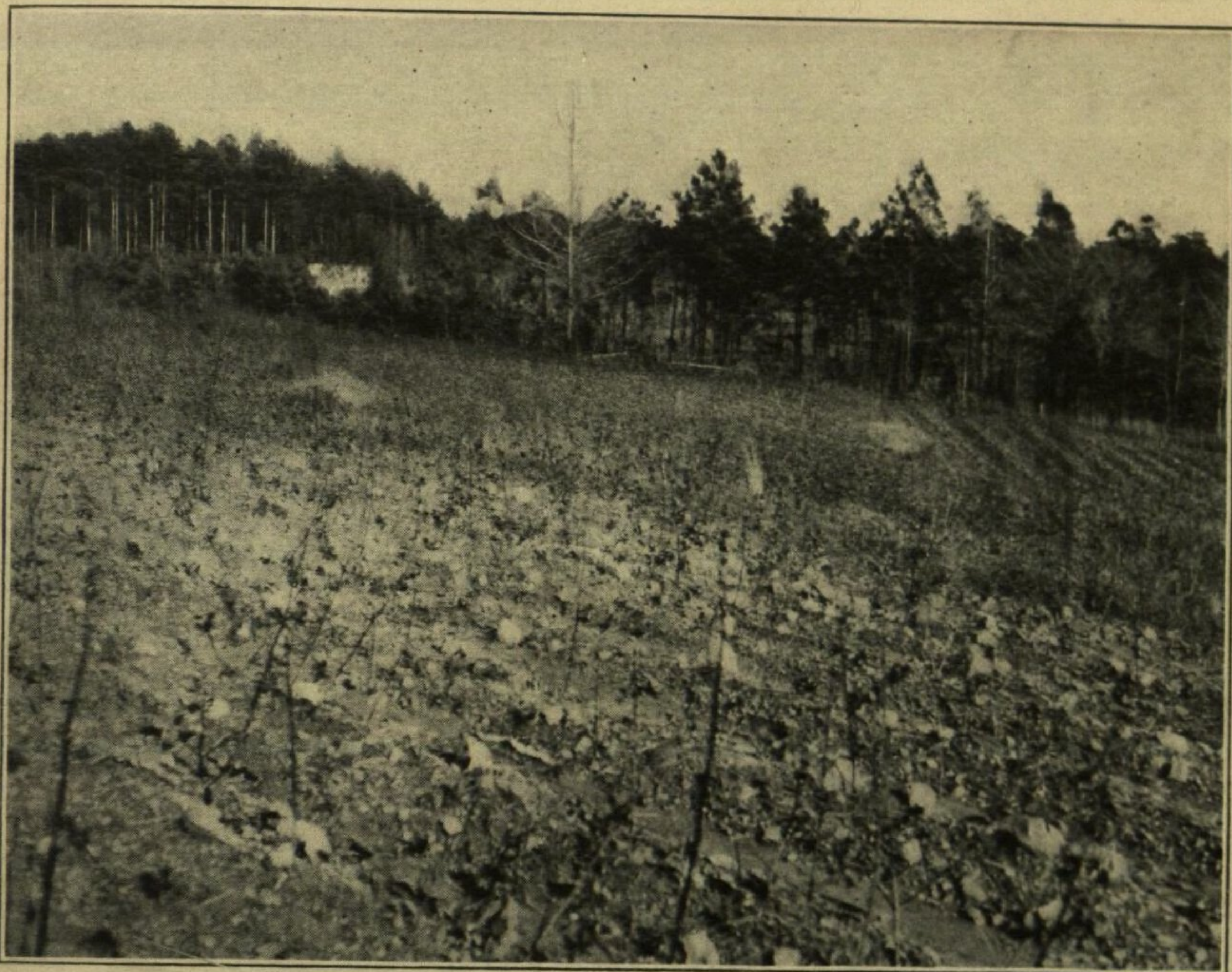
A.—Thin veneer of materials from the Lafayette formation consisting of smoothly rounded pebbles and cobbles in a matrix of coarse sand, resting on closely underlying, deeply decayed, crystalline rocks near Samaria, Unionhope road, 1\frac{1}{4} miles southwest of Samaria, Nash County, N. C.
