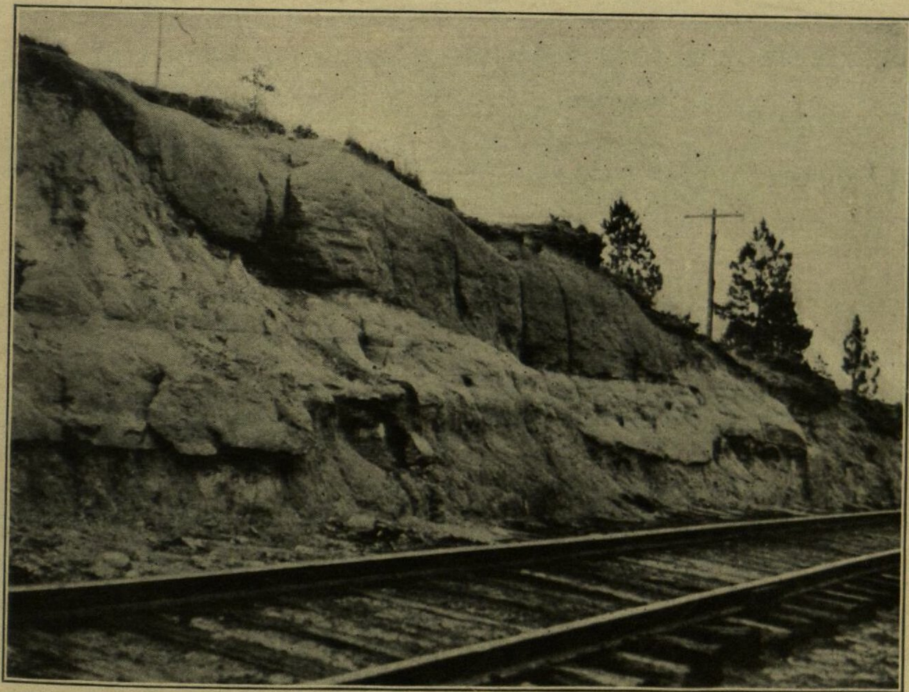
B.—Exposure of the Lafayette formation resting unconformably upon the Patuxent formation; cut of Seaboard Air Line Railway, 1 1-3 miles southwest of Lake View, Moore County, N. C.
