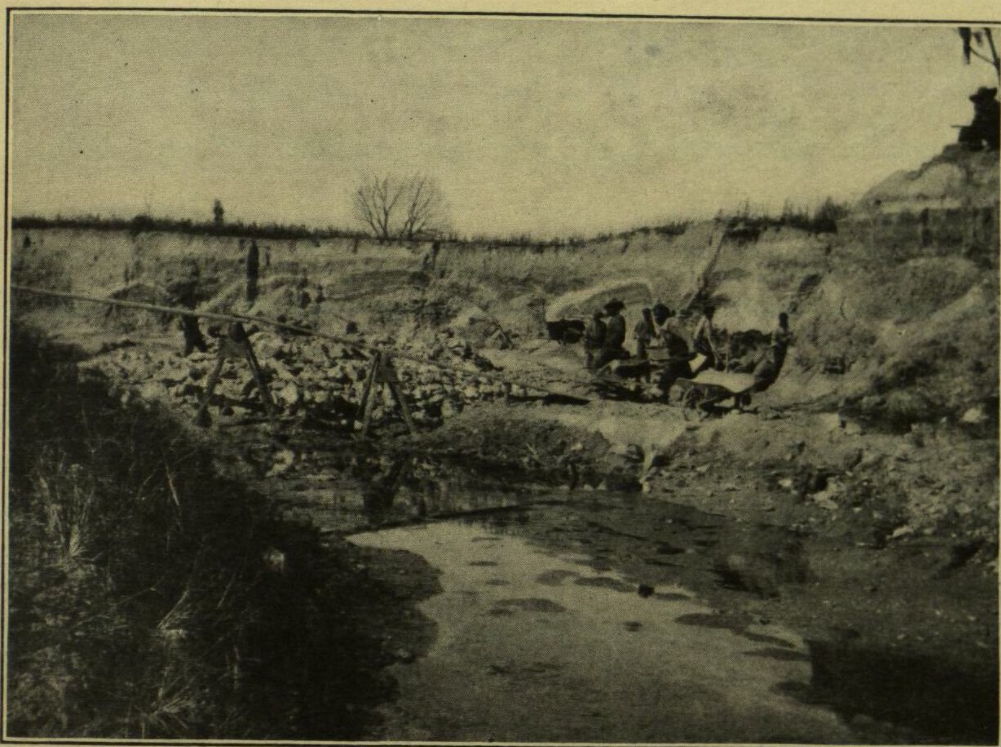
A.—Exposure of the Castle Hayne formation in the rock quarry near Castle Hayne, New Hanover County, N. C.
