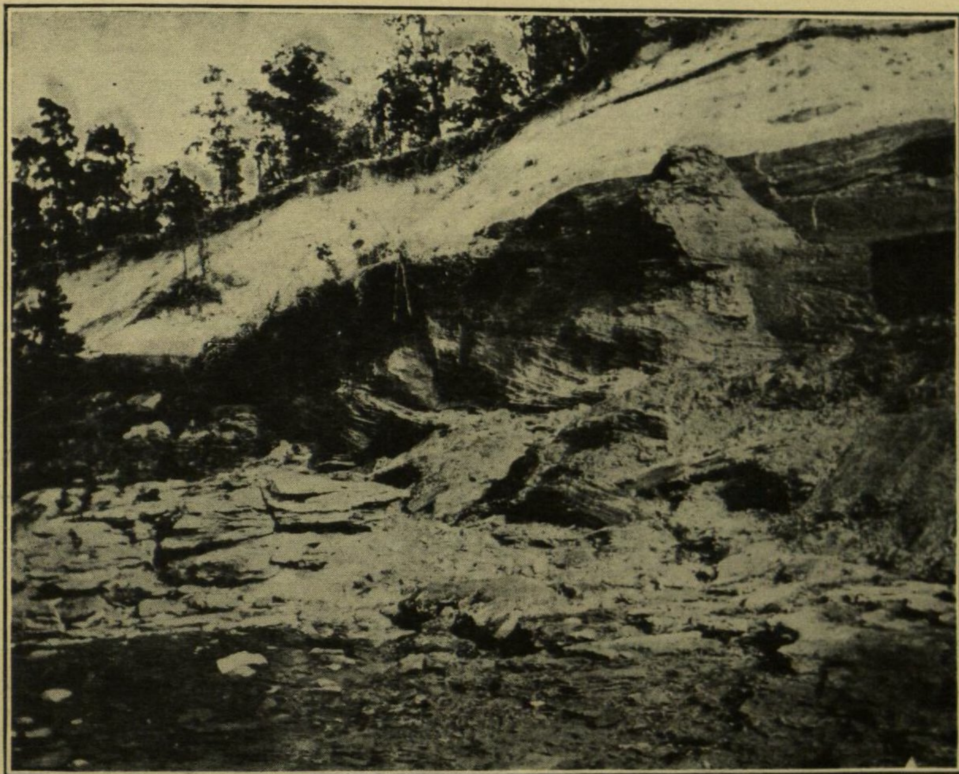
A.—Exposure of strata typical of the Black Creek formation overlain by white sands of Pleistocene age, Cape Fear River, Sand Bluff Landing, 3\frac{1}{2} miles below Elizabethtown, N. C.
