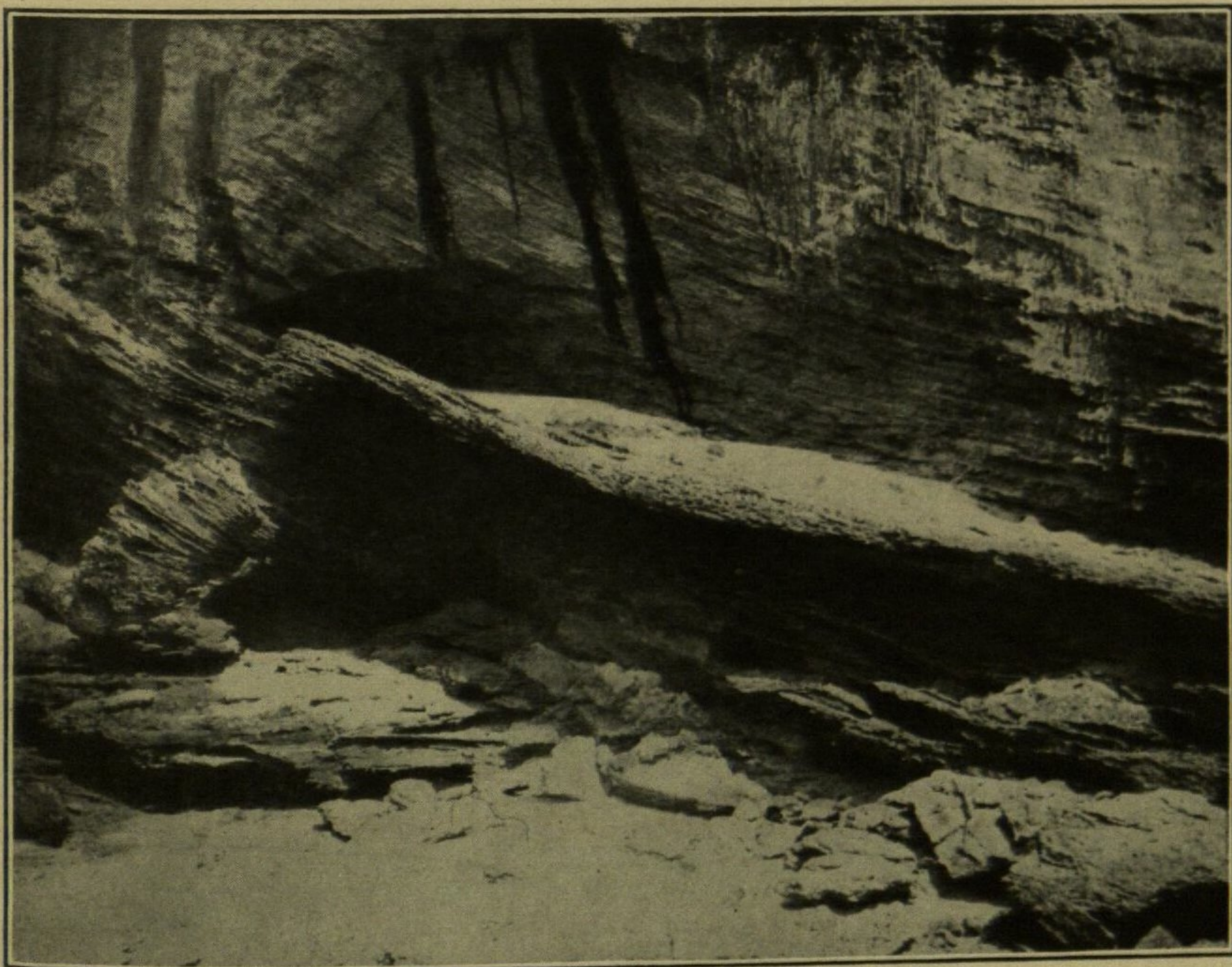
B.—Near view of laminated sands and clays typical of the Black Creek formation, Cape Fear River, Big Sugar Loaf Landing, 7\frac{1}{2} miles below Elizabethtown, N. C.
