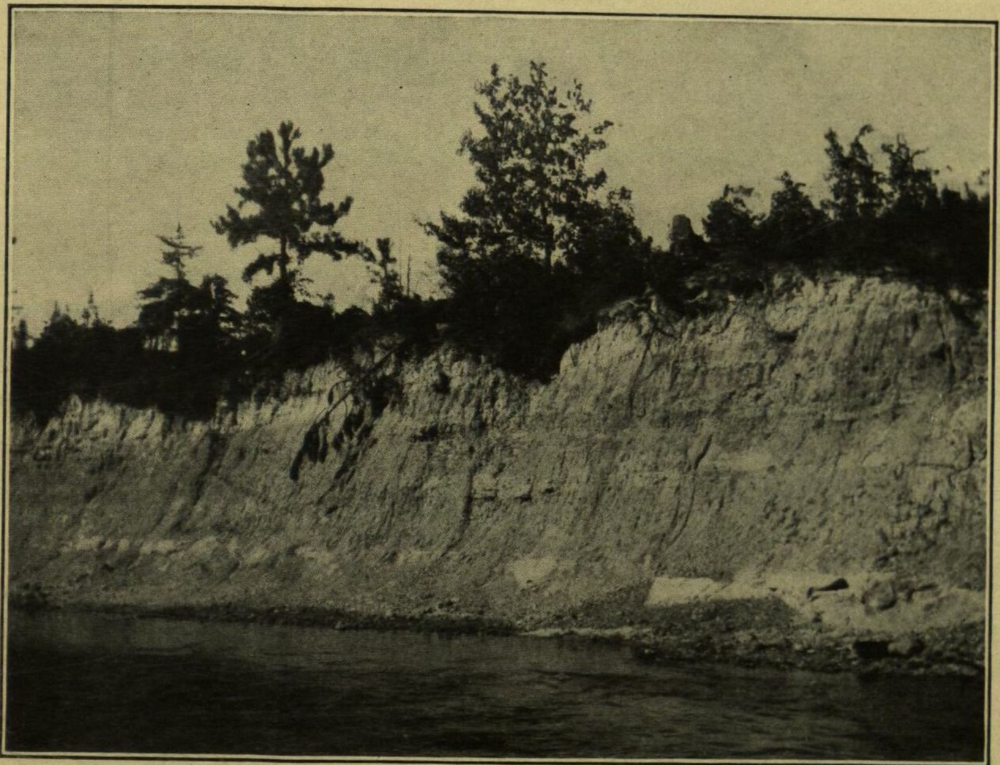
A.—Exposure of the Patuxent formation, Little River, one-half mile below the railroad bridge at Manchester, Cumberland County, N. C.
