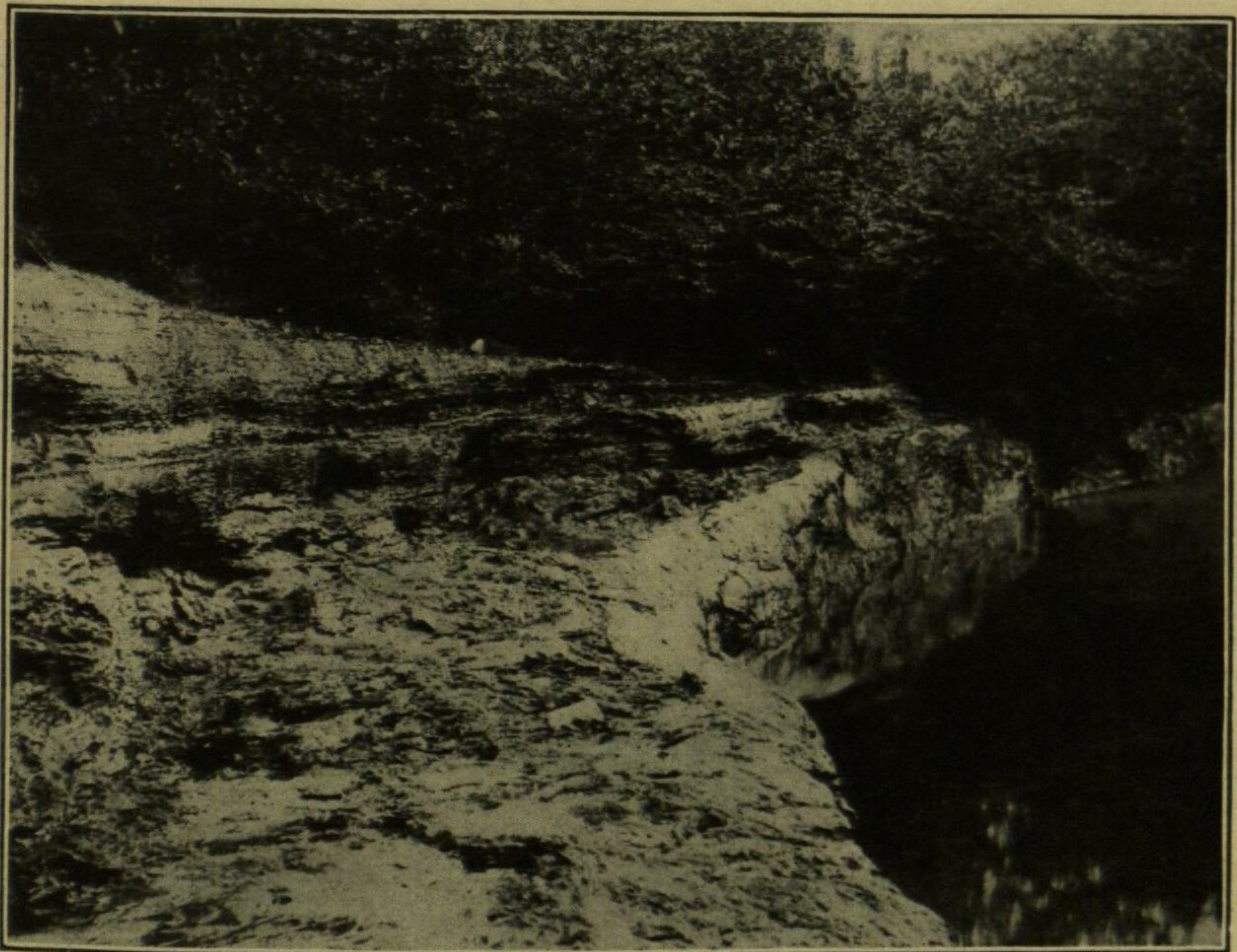
B.—Exposure on Neuse River at county bridge, two miles southwest of Goldsboro, N. C. Shows unconformable contact between the Patuxent and Black Creek formations.
