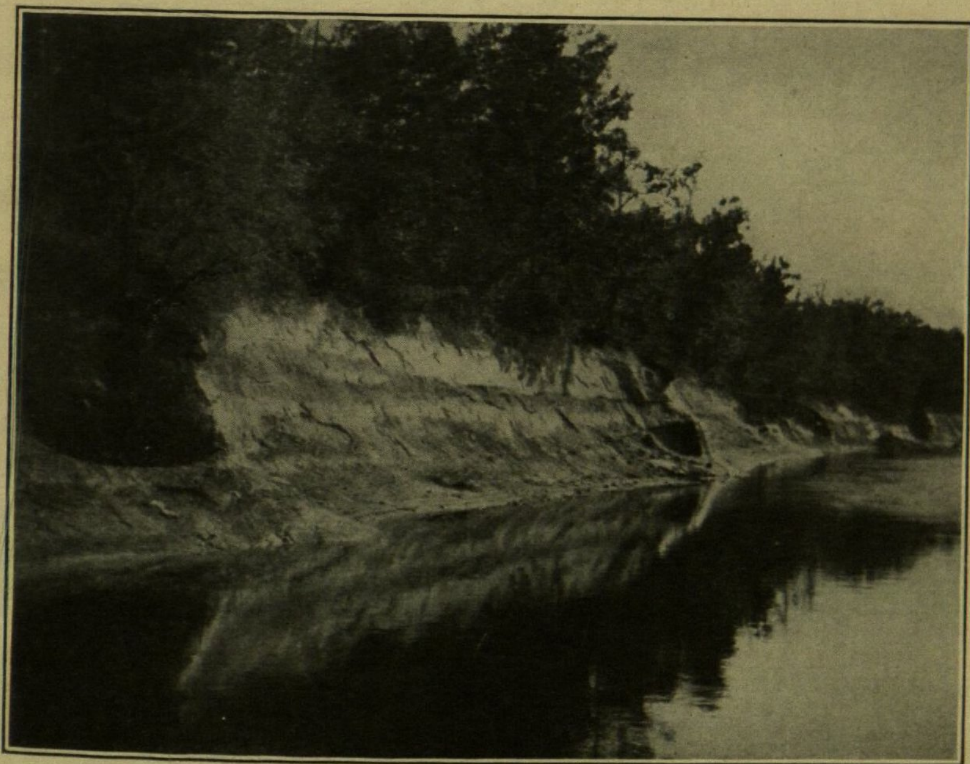
B.—Exposure of the Patuxent formation, Cape Fear River, about 10 miles below Fayetteville, N. C. Shows also the projections described on page 91.
