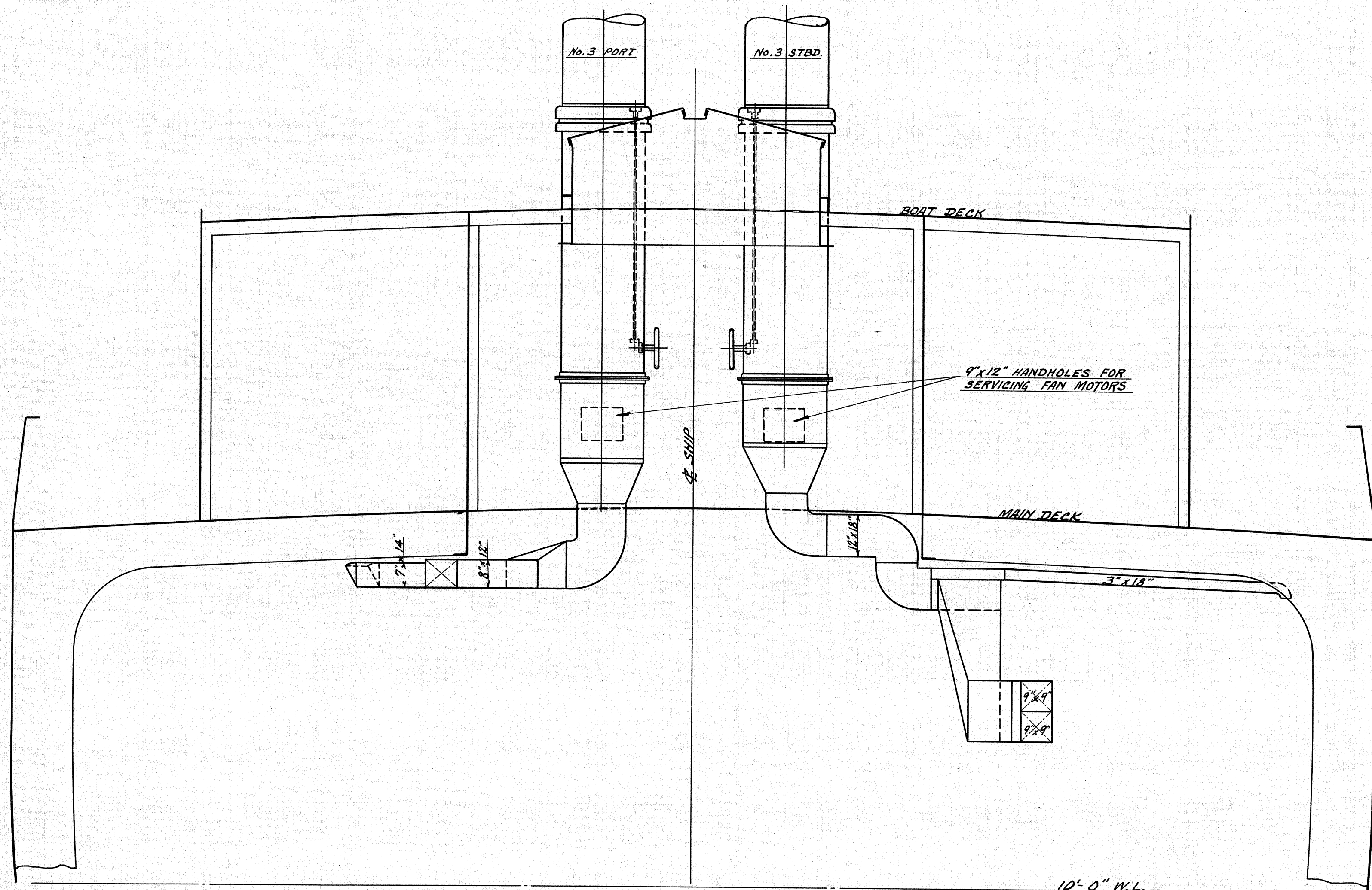
SECTION AT FR. No. 18 LOOKING FWD.
