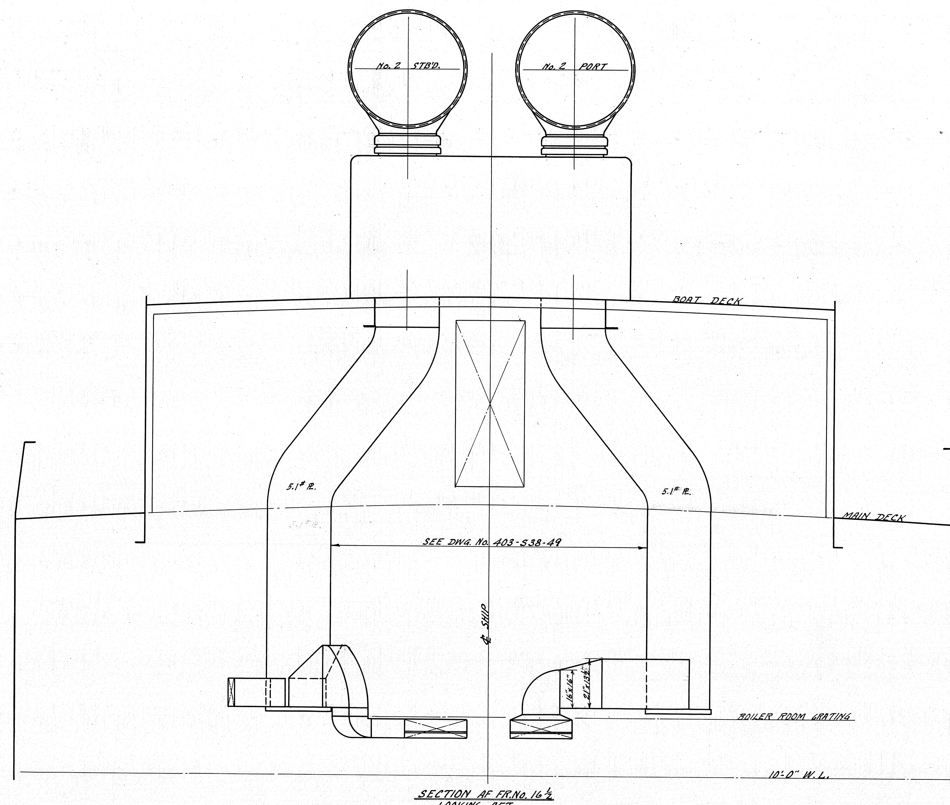
SECTION AT FR. No. 16 1/2 LOOKING AFT.
