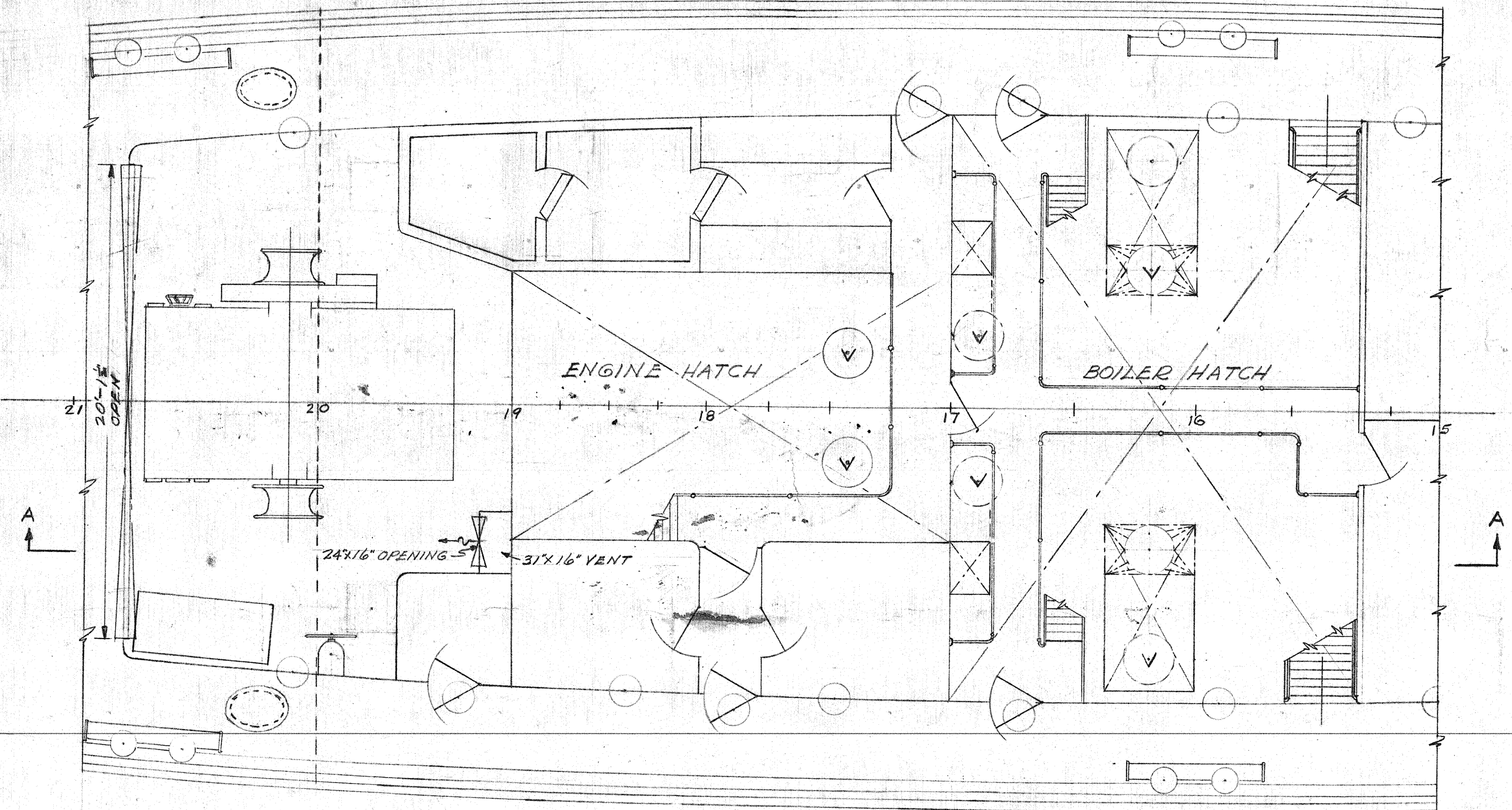
MAIN DECK SCALE 1/4" = 1'-0"
