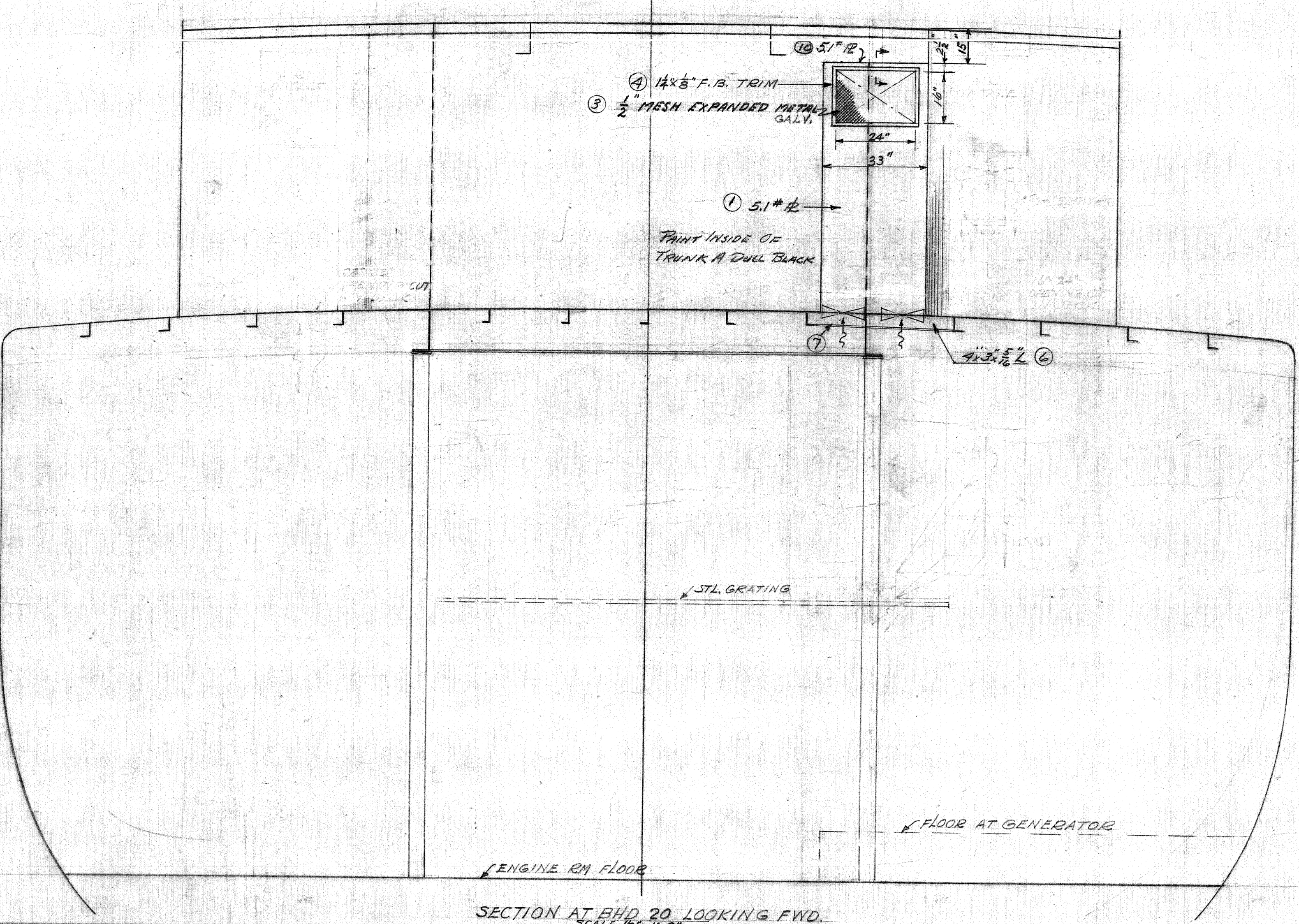
SECTION AT BHD 20 LOOKING FWD. SCALE 1/2" = 1'-0"
