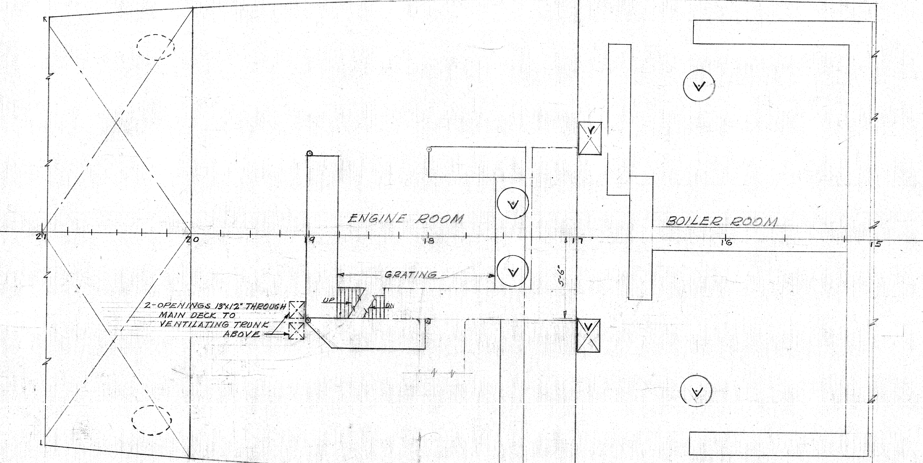
PLATFORM DECKS SCALE 1/4" = 1'-0"
