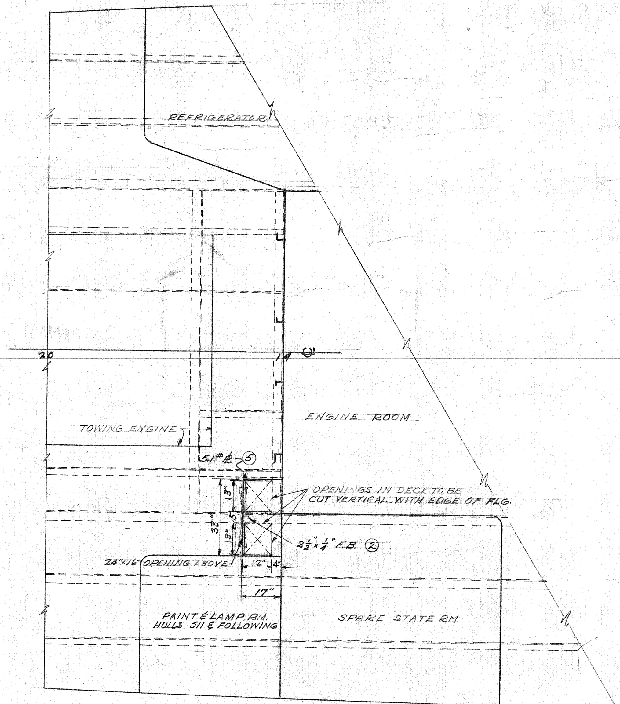
PLAN AT MAIN DECK SCALE 1/2" = 1'-0"
