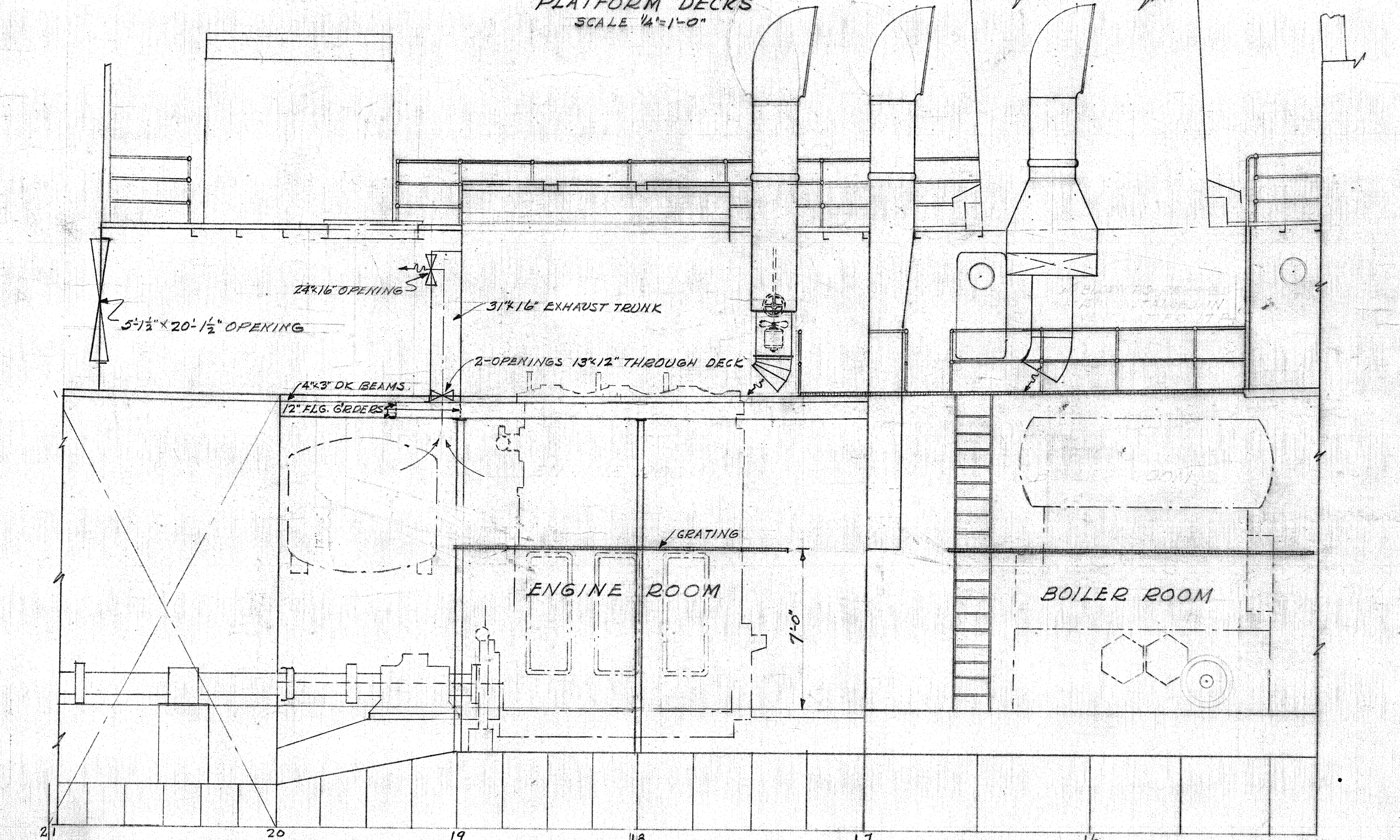
PROFILE SECTION THROUGH ENGINE & BOILER ROOMS AT A-A SCALE 1/4" = 1'-0"
