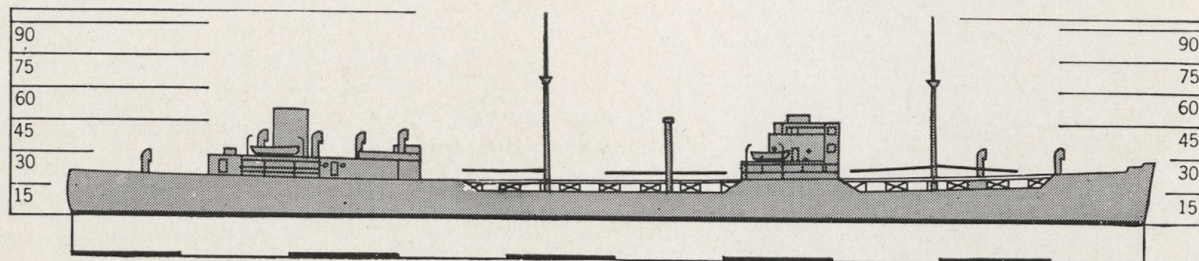
TEIYO MARU—XAO 11
