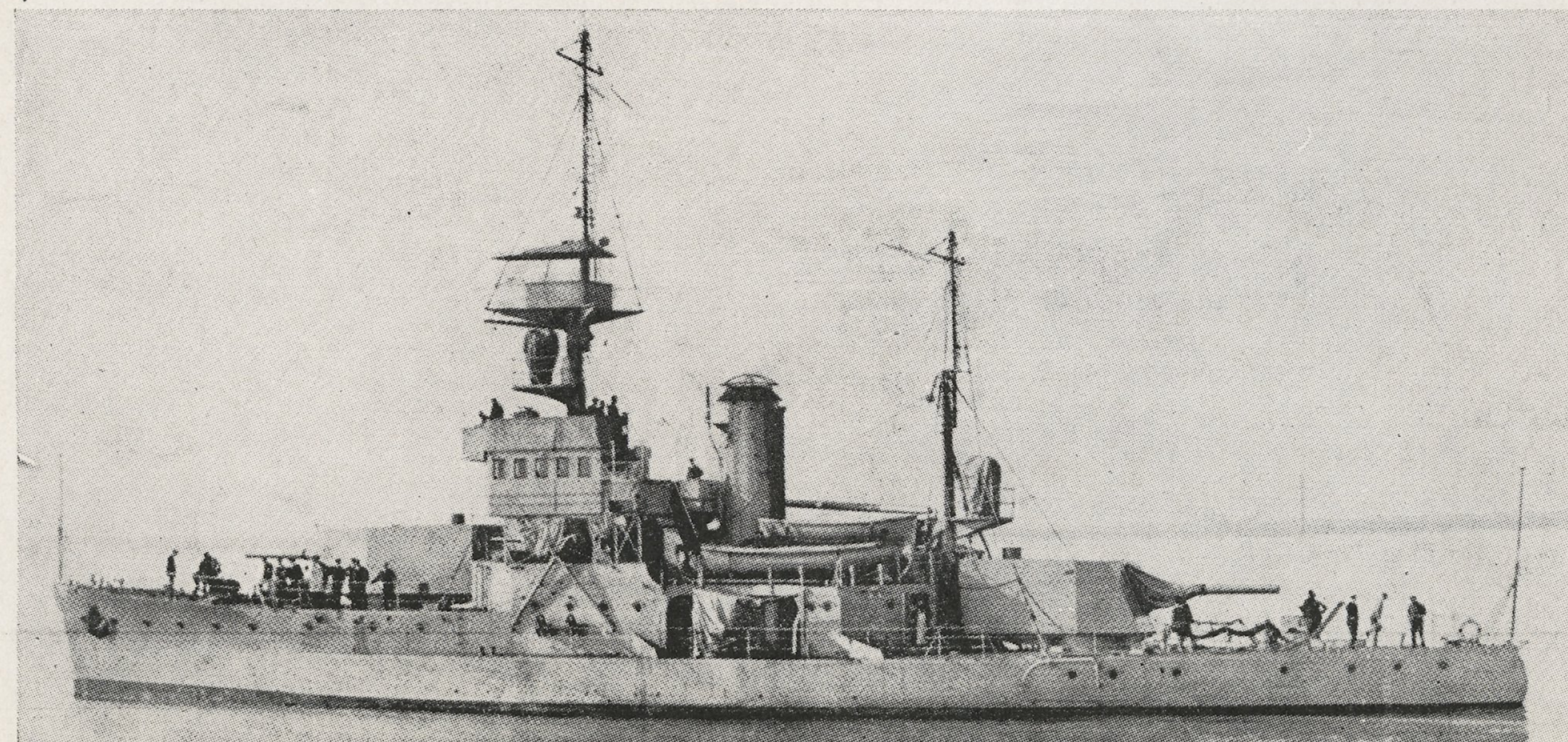
↓ SUKHODAYA—CD-2—FOREMAST SINCE LOWERED, MAINMAST HEIGHTENED.
