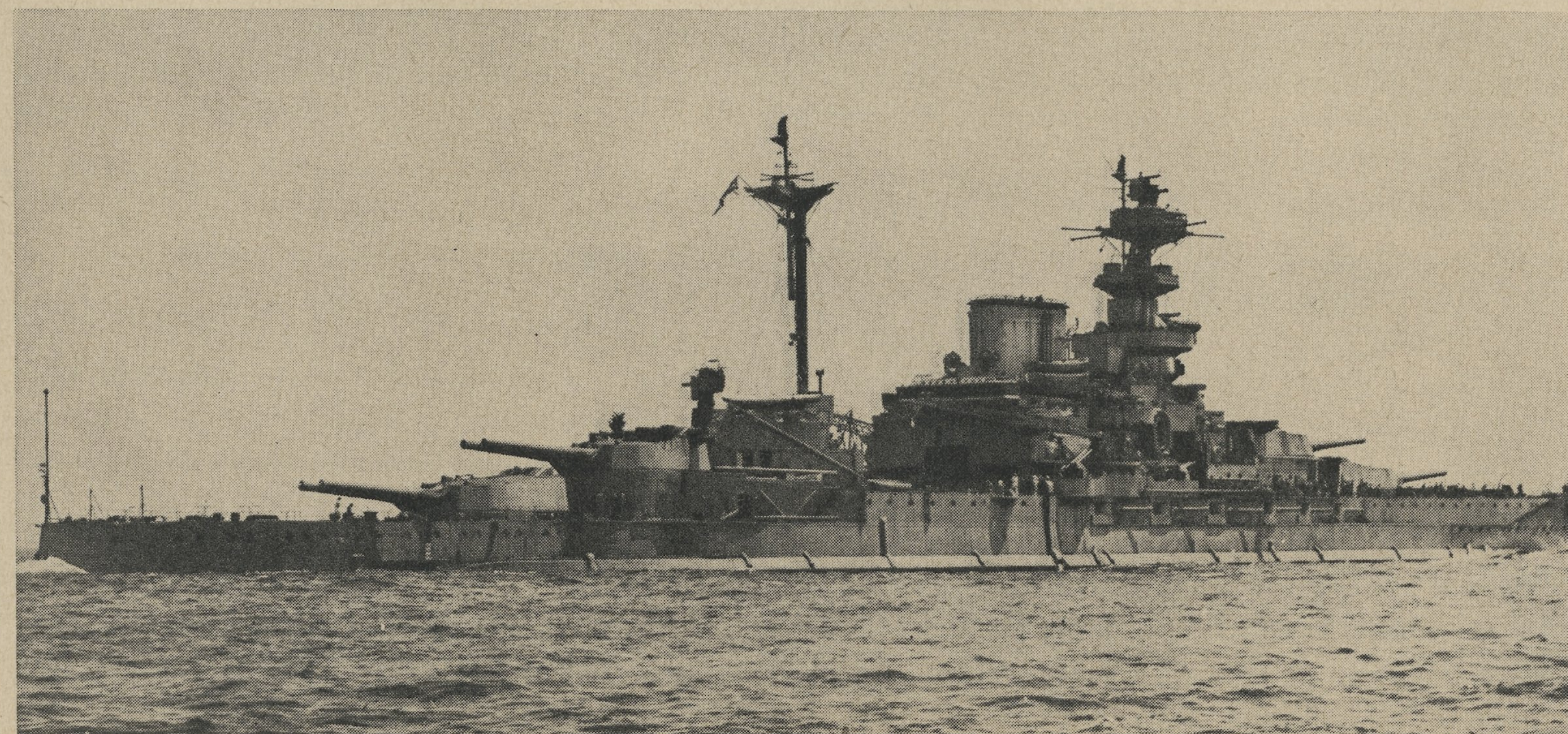
MALAYA —note aircraft hangar abaft stack.
