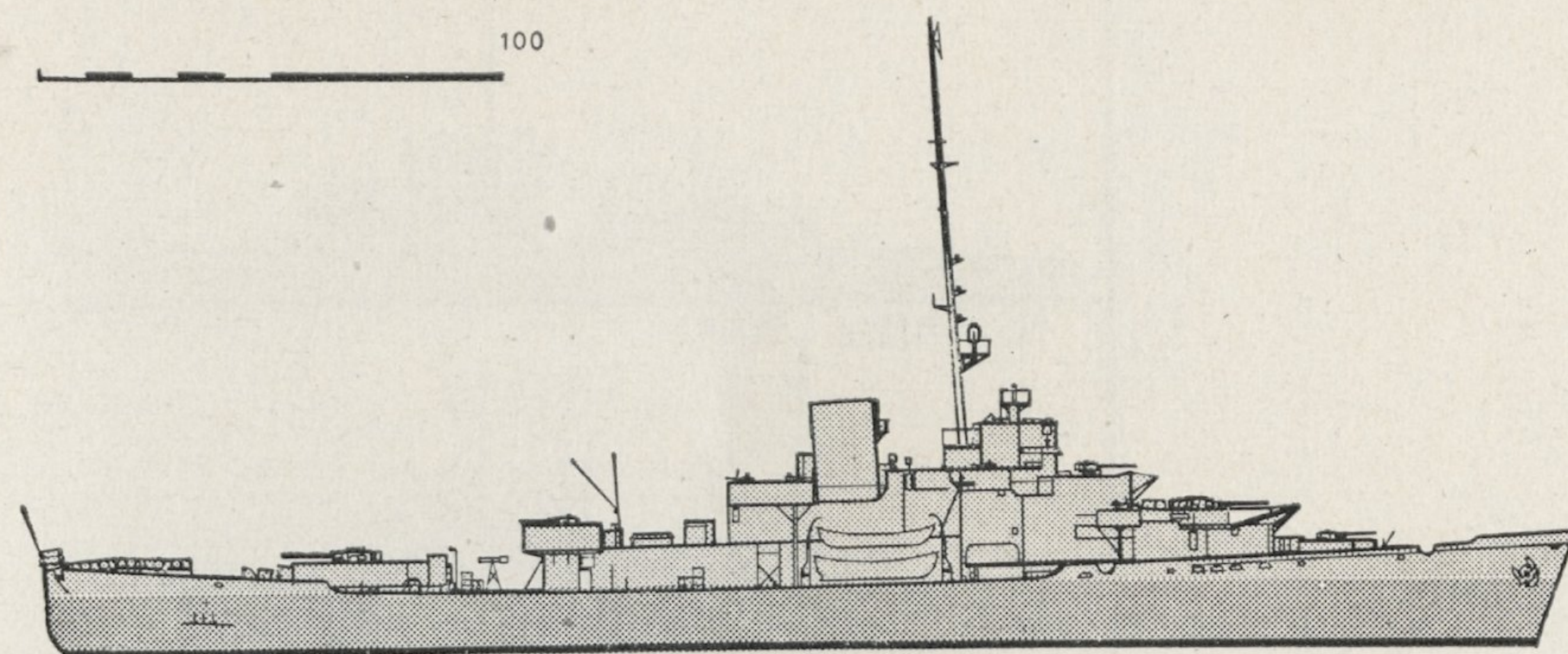
PG—COAST GUARD CUTTER
