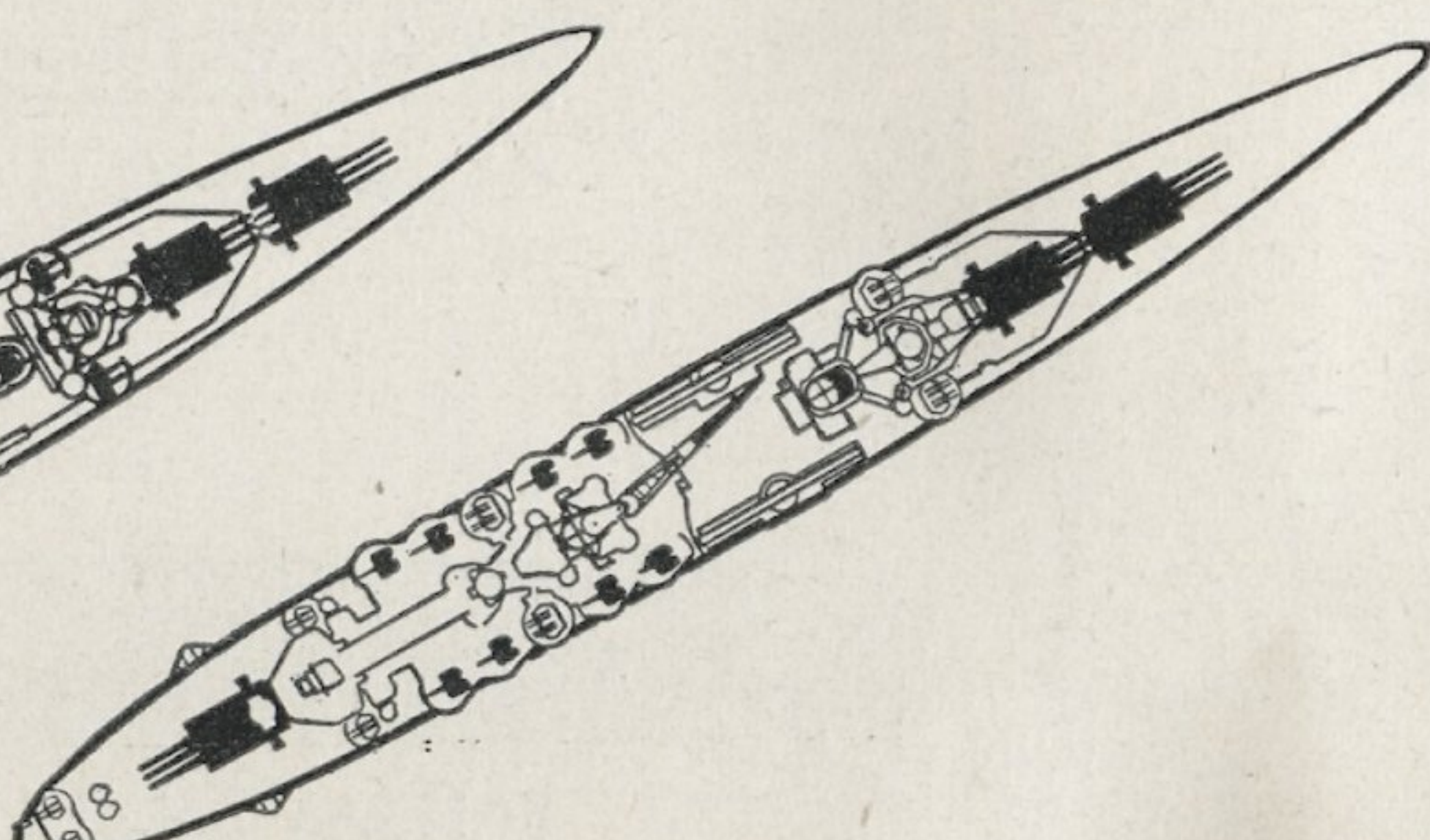
NORTHAMPTON
