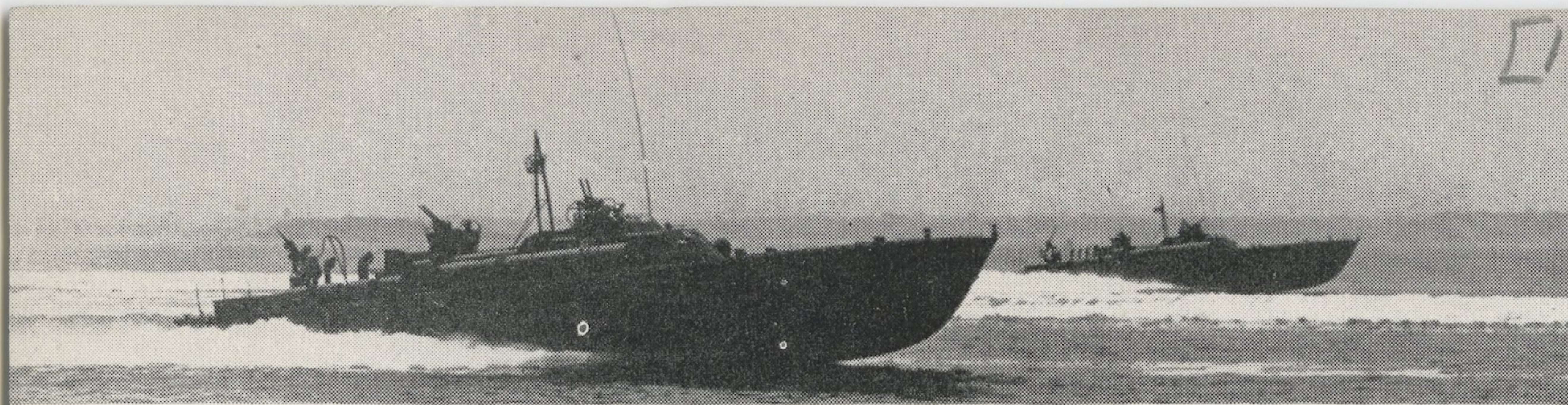
▲ PT 103 Class, shown during high-speed trials. Note variance in armament and torpedo layout—also new radar.
