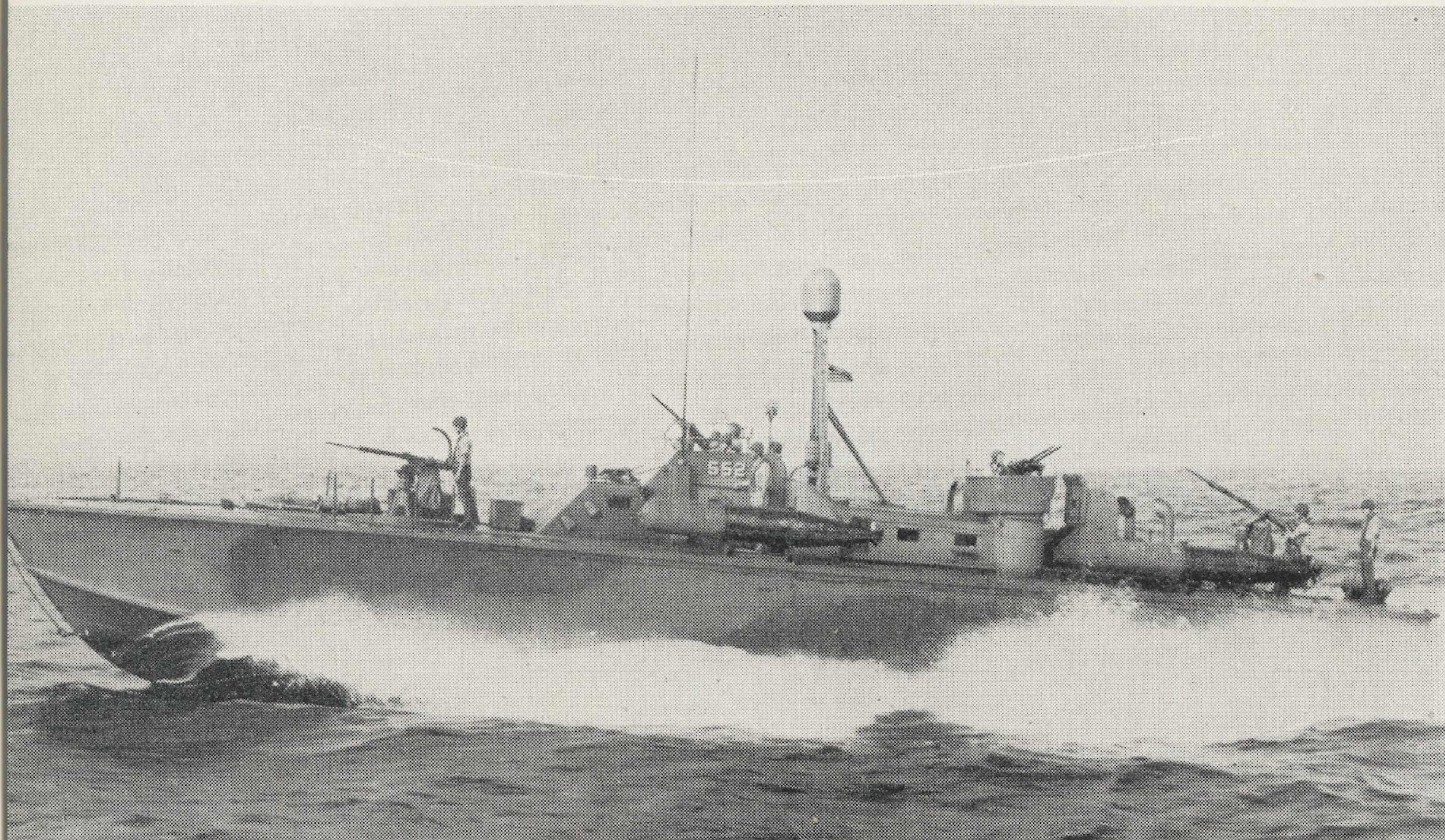
▼ PT 103 Class, showing typical torpedo boat hull shape.
