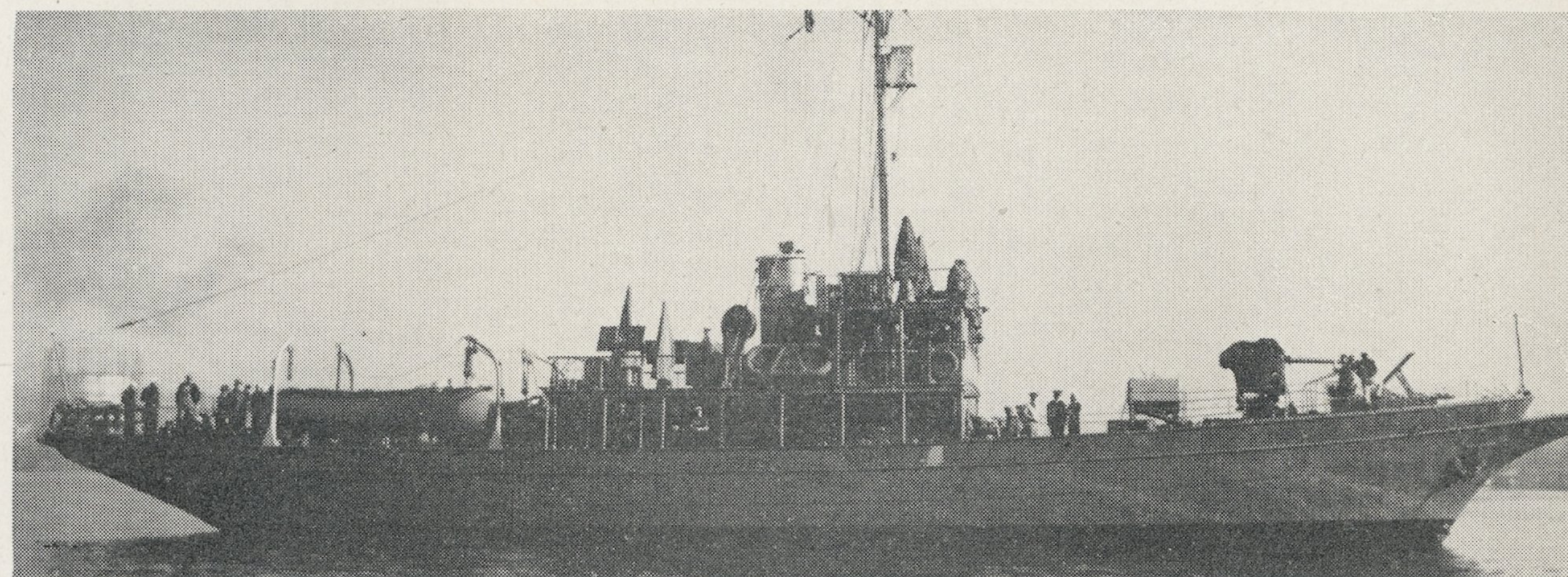
▲ PYc 45—BLACK DOUGLAS. Length, 153 feet. Photo 3-30-43.
