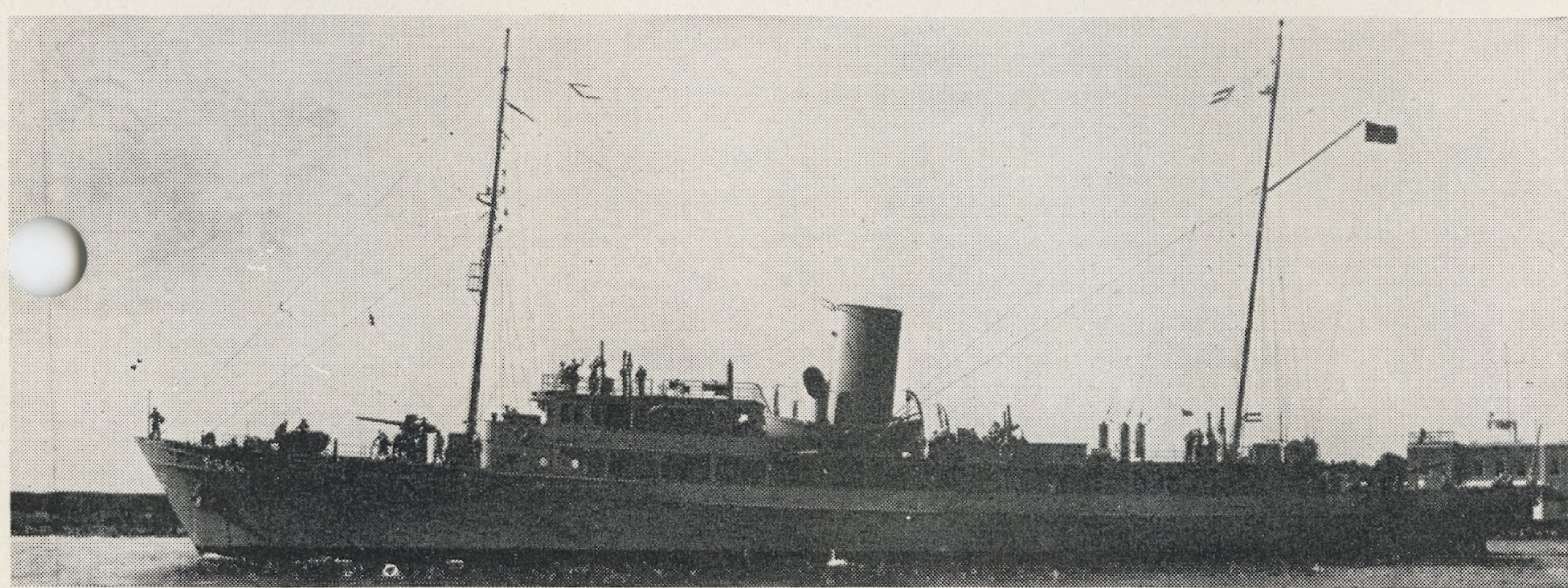
▲ PG 60—BEAUMONT, ex-yacht CAROLA. Length overall, 226 feet. ▼ AGP 3—JAMESTOWN, ex-PG 58. Length overall, 294 feet.
