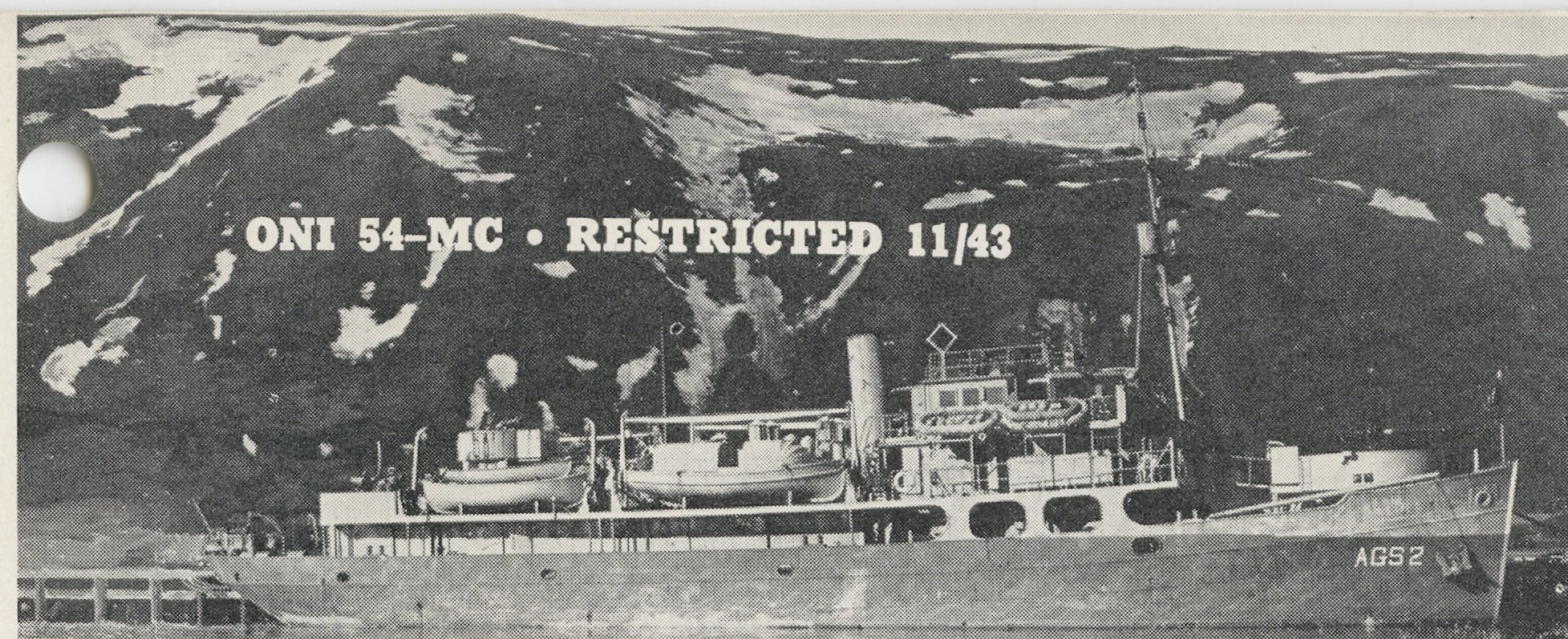
▲ AGS 2—HYDROGRAPHER, a surveying ship. Length overall, 164 feet.
