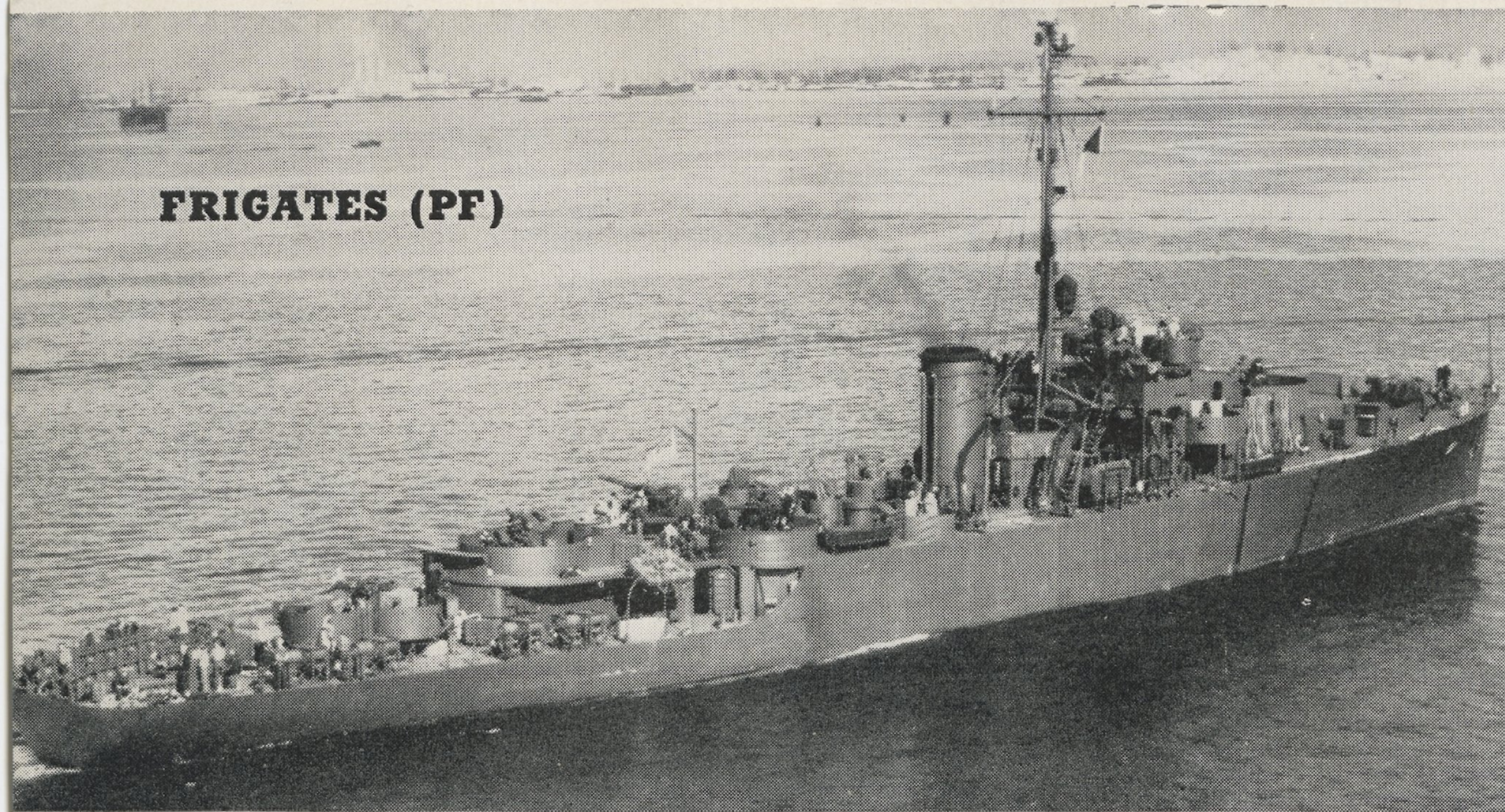
▲ PF 37—SAN PEDRO and PF 2—NATCHEZ ▼ illustrate the destroyer-like appearance of this design. Note hull is broken aft, and that stack is not supported by any superstructure.
