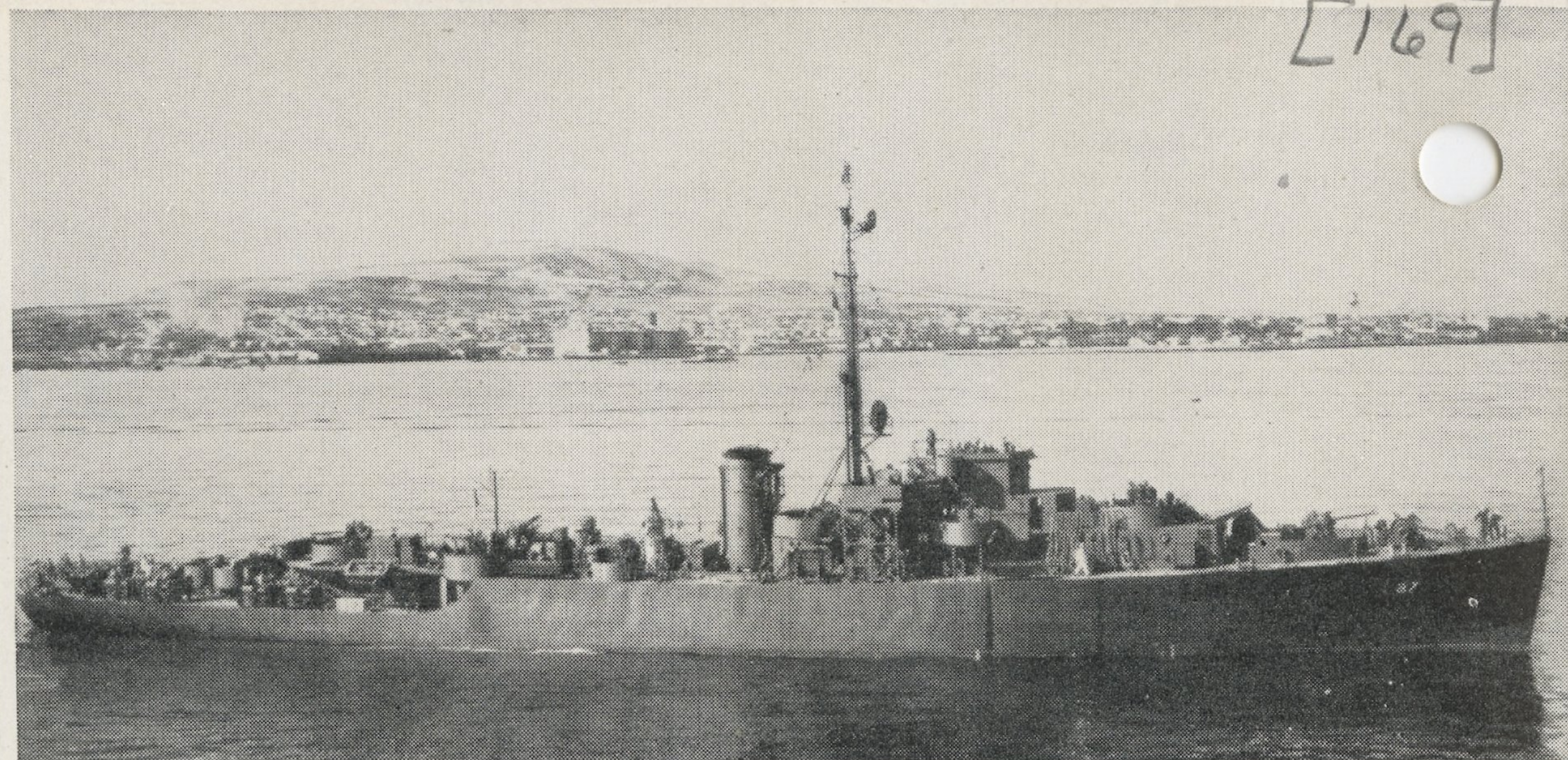
▲ PF 37—SAN PEDRO and PF 2—NATCHEZ ▼ illustrate the destroyer-like appearance of this design. Note hull is broken aft, and that stack is not supported by any superstructure.
