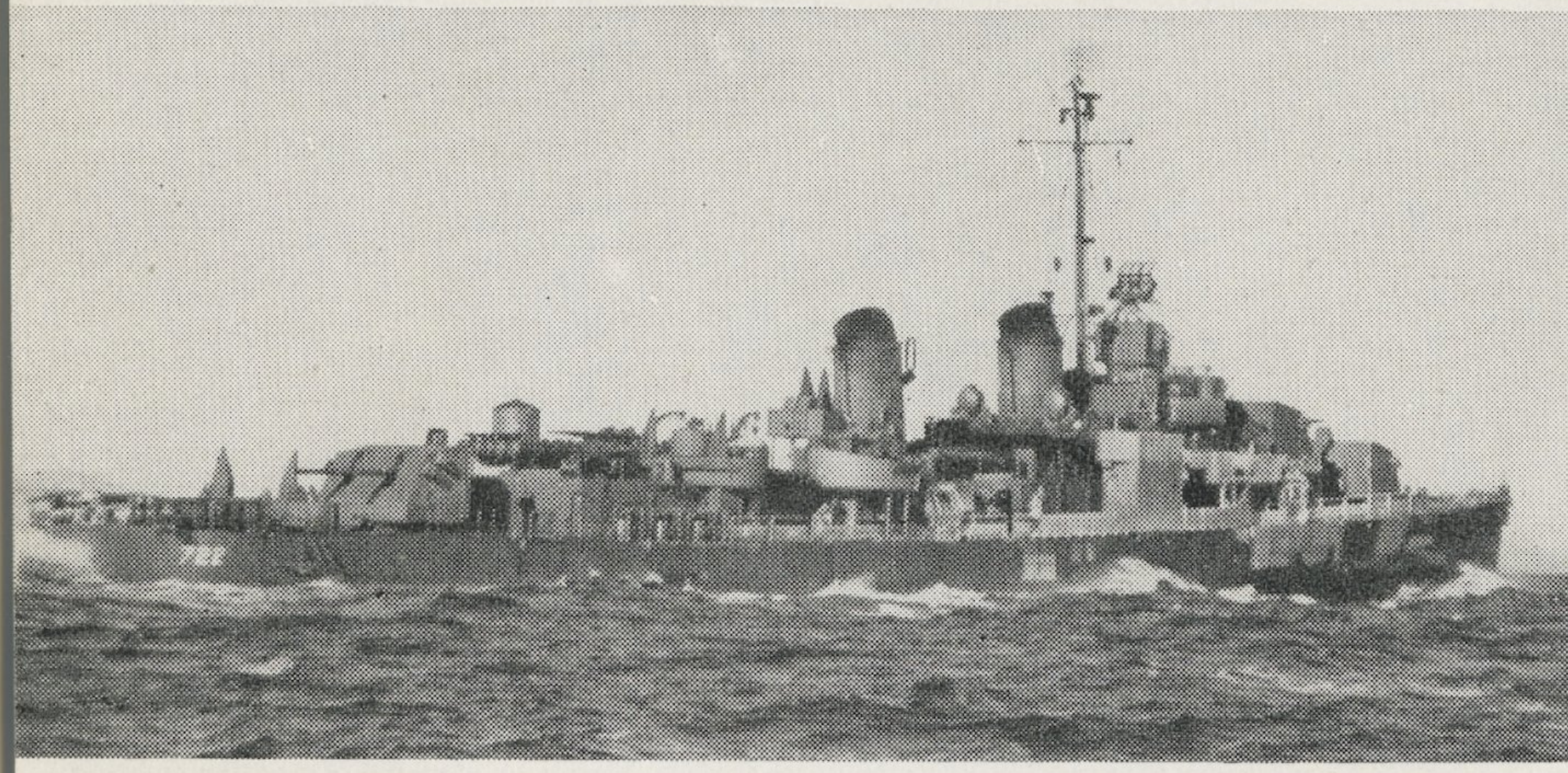
The twin 5"/38 mounts illustrated also form the standard secondary battery seen on all our new BB's, CA's, and CL's. All photos are of the BARTON, taken 12-29-43.
