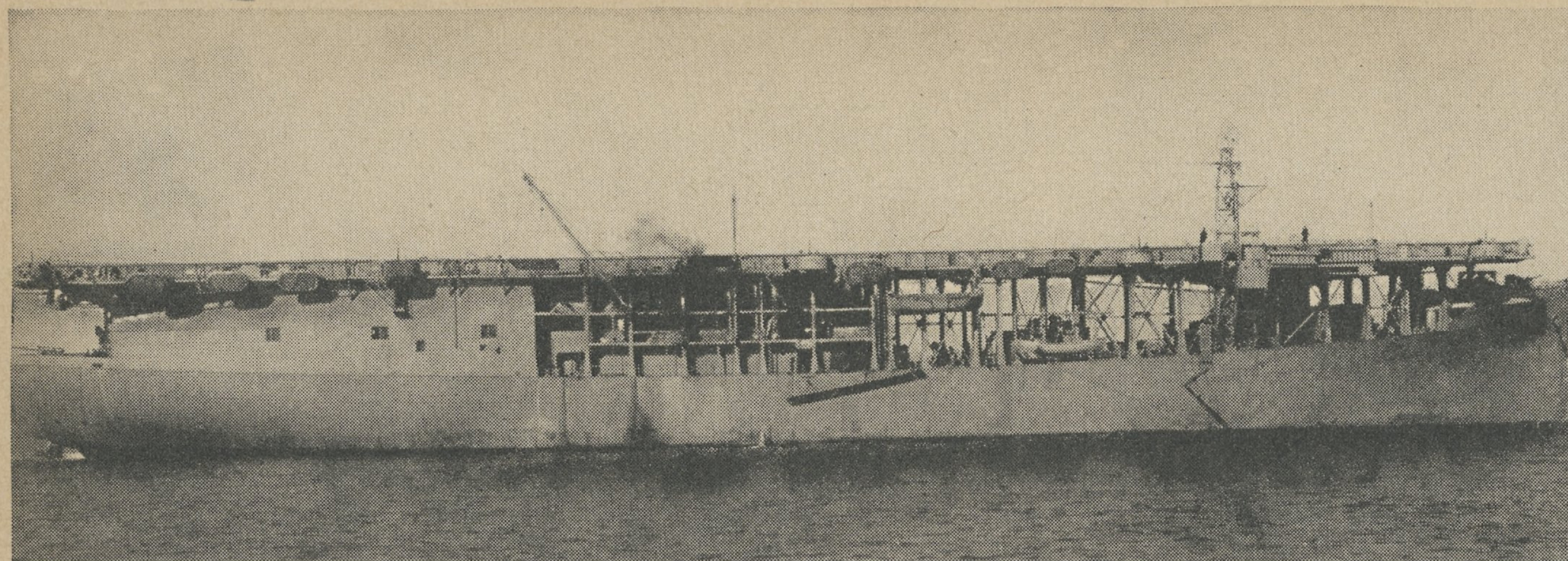
▲ British sister ship to the LONG ISLAND, HMS ARCHER, 12-41. All photographs of the LONG ISLAND, 12-19-42; of CHARGER, ▼ 9-24-42.
