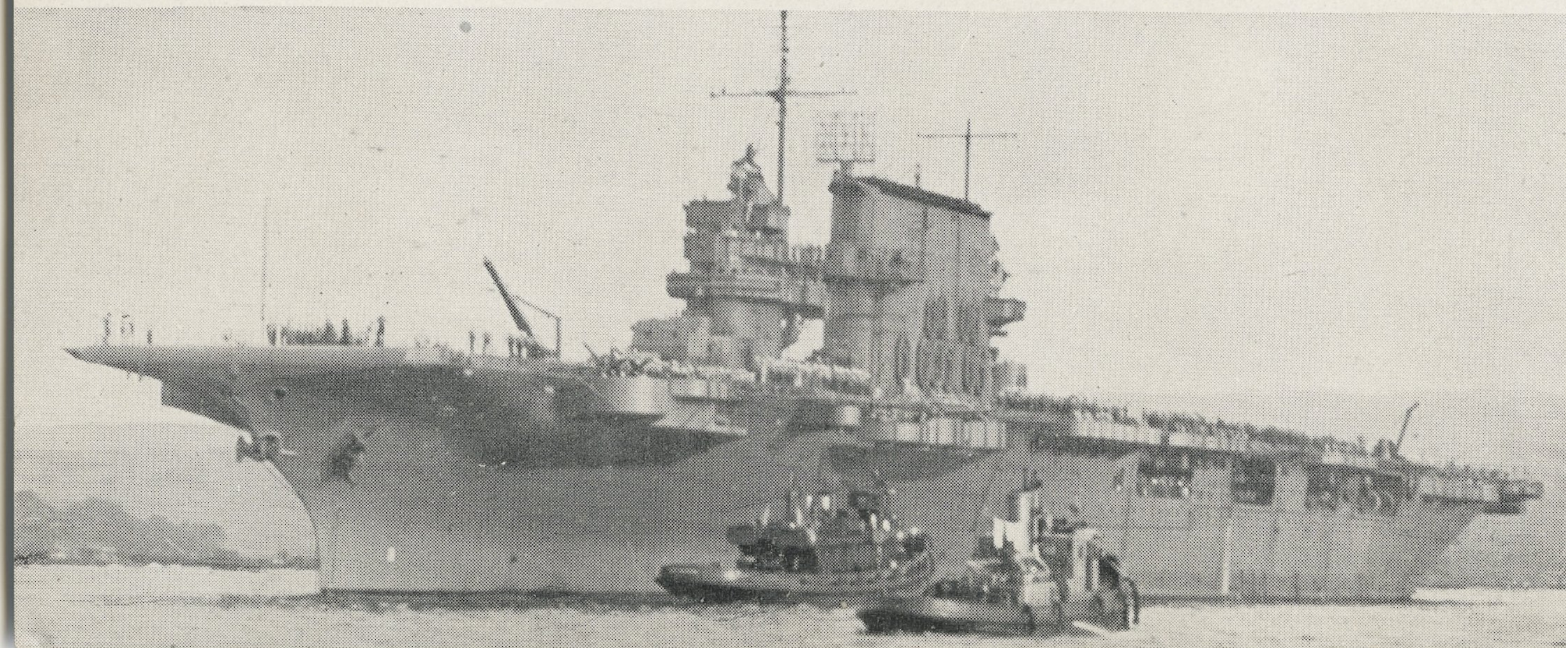
▲ Photos 11-6-42 showing new 20 and 40 MM machine gun positions, and other minor superstructural alterations. ▼
