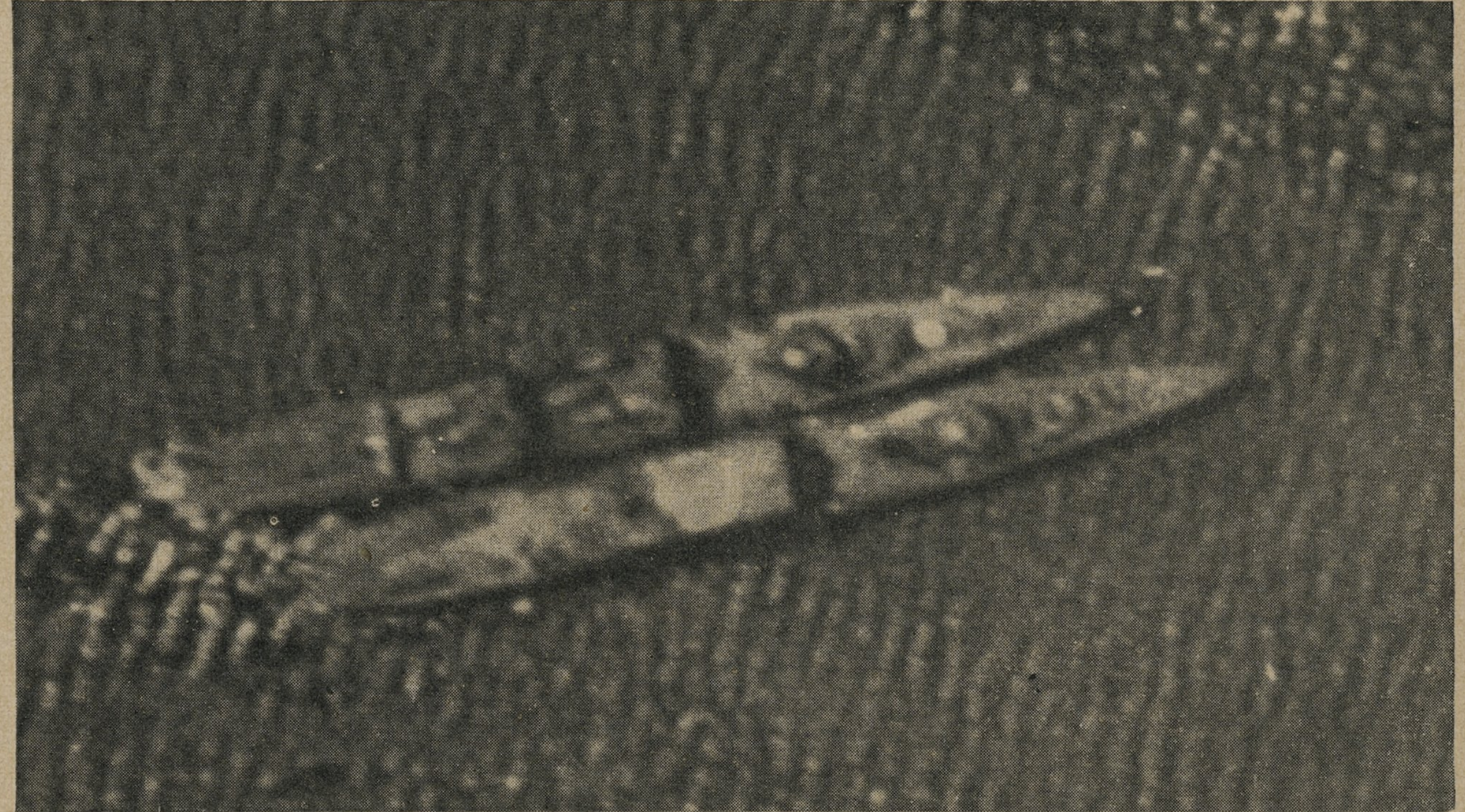
A CHITOSE Class seaplane tender. Note the identification ring amidships. Compare with MIZUHO Class above and on opposite page. The aircraft handling trusses are roofed over in this ship and the stack is abaft the bridge.
