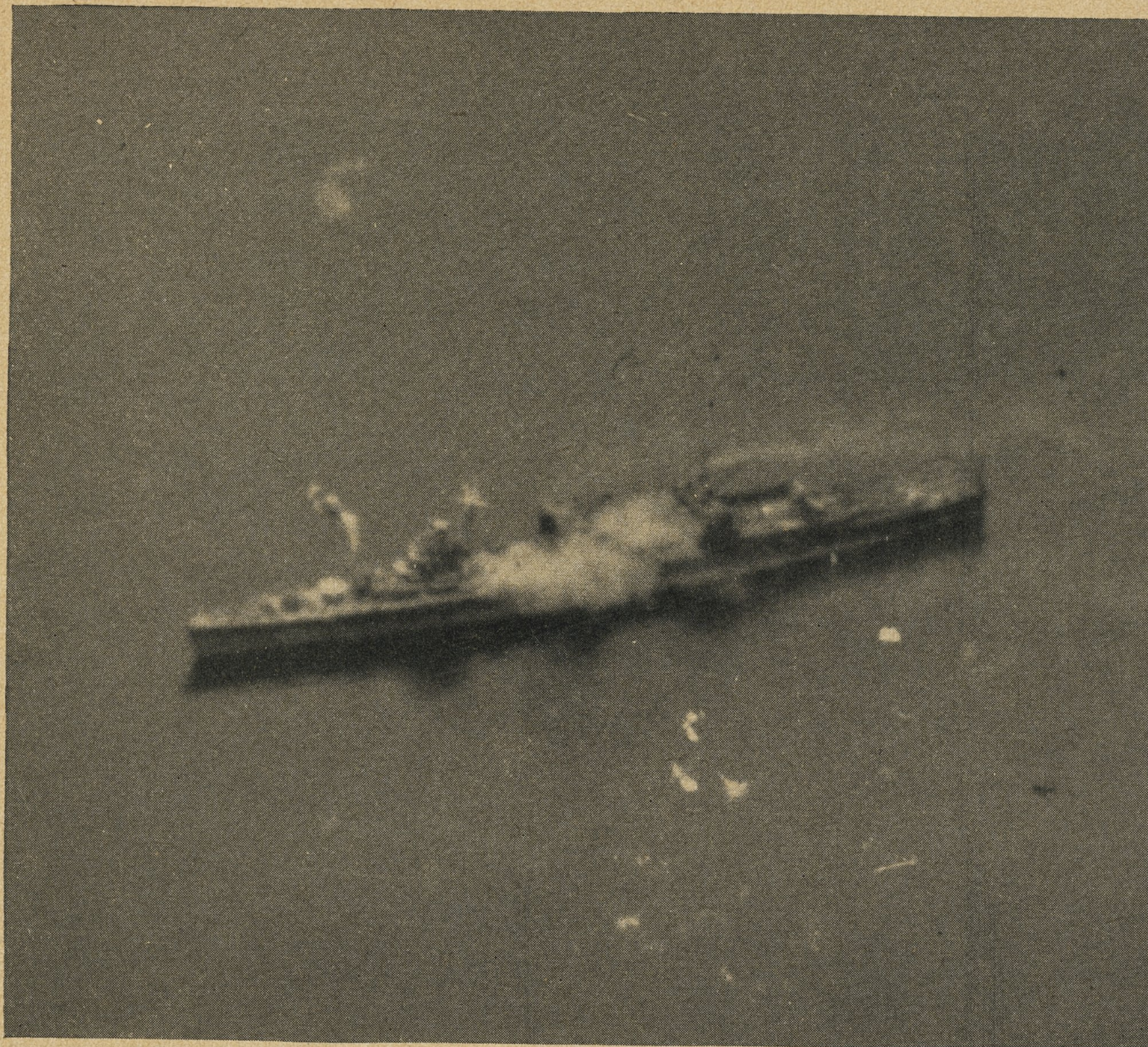
Seaplane tender of the MIZUHO Class. The photograph at the right shows clearly the strong transverse shadows cast by her plane handling trusses. Compare with plan alongside for gun location and bridge structure.
