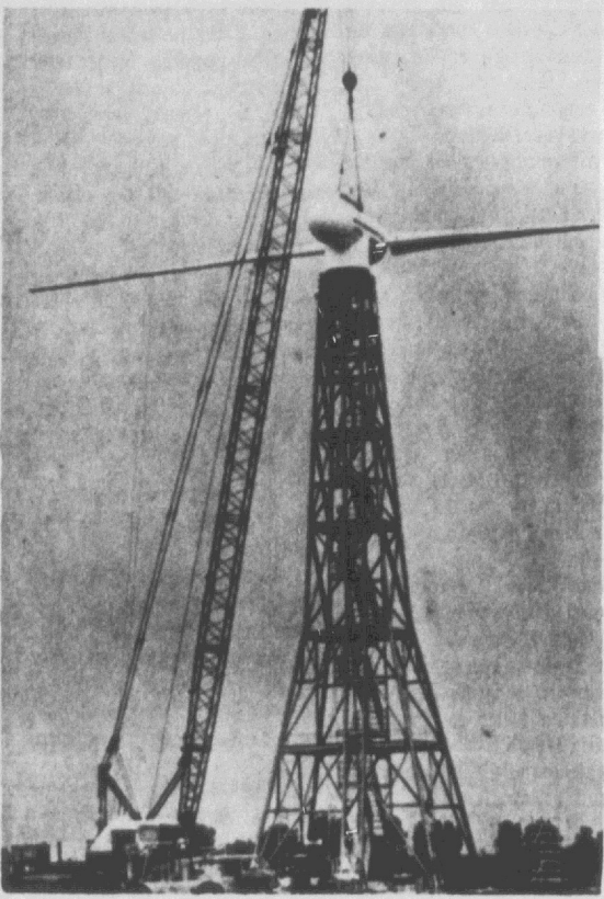
EXPERIMENTAL SOURCE —National Aeronautics and Space Administration engineers mounted the blades for an experimental windmill, hoping they would be a source of energy. The windmill is located near Sandusky Ohio. (AP Wirephoto)
