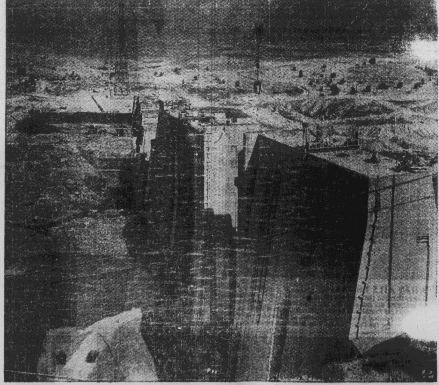
CONQUERING THE WILD CANADIAN RIVER , the $16,240,000 Conchas dam in New Mexico—largest dam project in the southwest—has for its main unit above 1,250-foot-long mass of concrete. Dam is key to a vast irrigation district.
