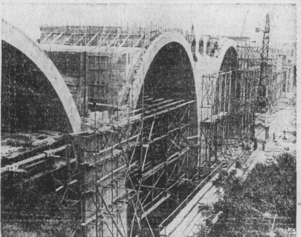
BRIDGE WITHOUT STEEL is being built near Jena by Germans who are using chalk. Sixteen pillars will support the arches. It is Germany's longest autoroad bridge.
