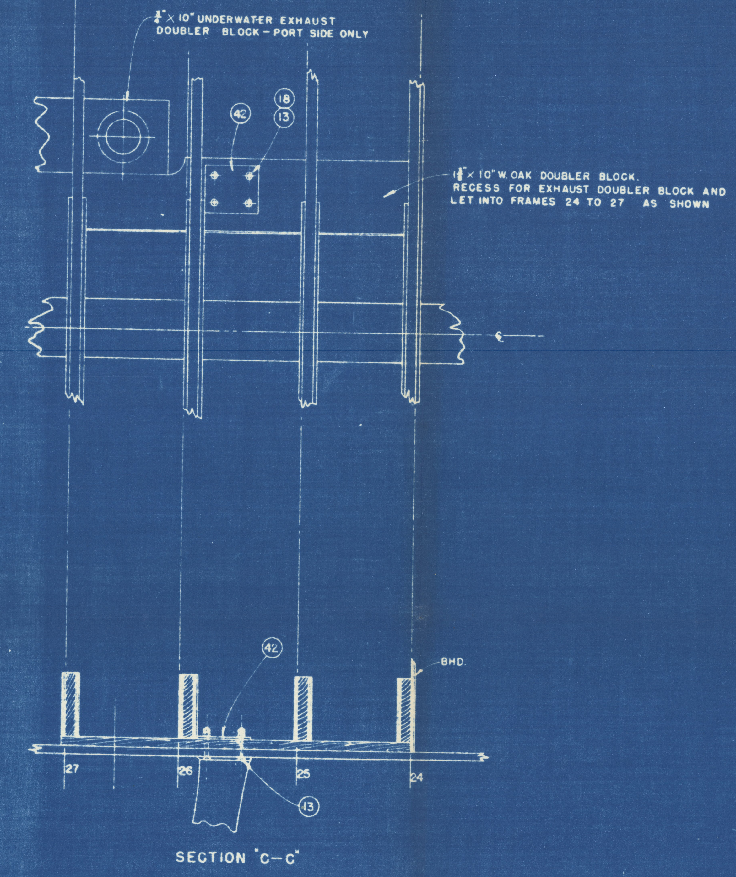
SECTION 'C-C'
