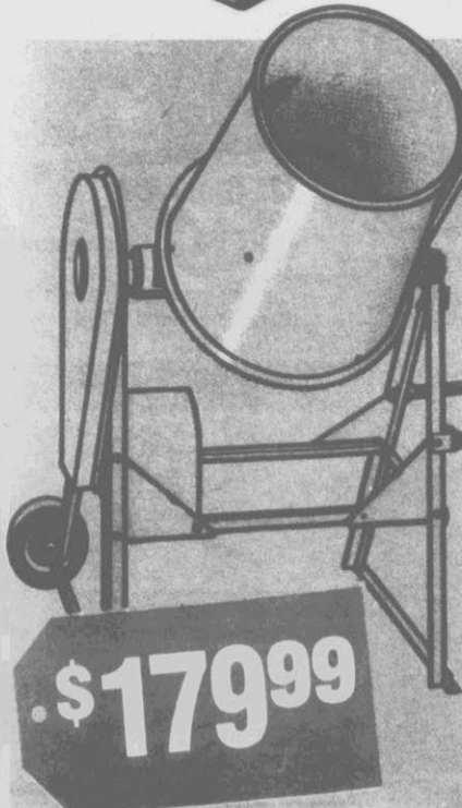
Cement Mixer Drum locks into place while mixing. 3.5 cu. ft. capacity drum. 1/2 HP motor. Cast iron drum base. #90197
