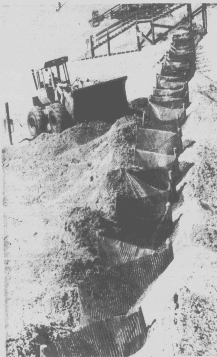
BEACH REBUILDING — A front end loader deposits sand from the Folly River behind a specially designed fence that officials hope will keep the sand at Folly Beach, S.C., from washing away. The project is taking place at the west end of Folly Beach near Charleston, S.C. (AP Laserphoto)
