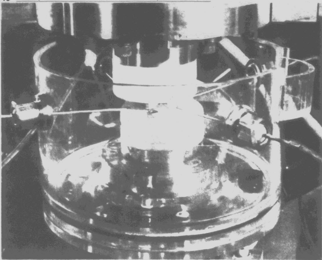
CHEWING MACHINE — University of Minnesota researchers at Minneapolis have built an artificial mouth that chews for hours and is used to test materials that could improve false teeth, bridges, crowns and fillings. (AP Laserphoto)
