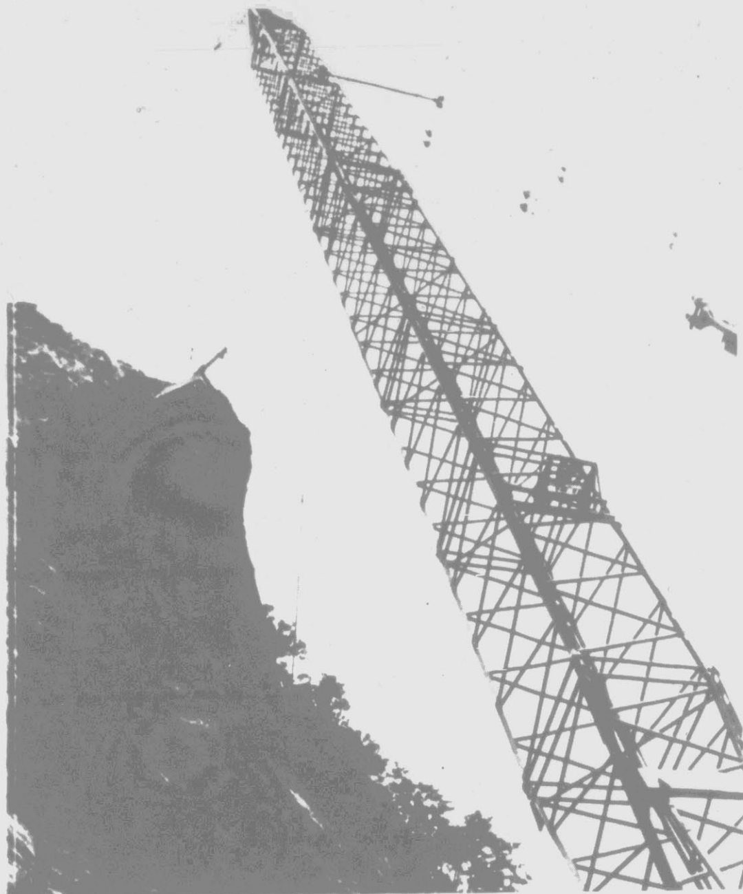
GLUE AND BOLTS — High in the Great Smoky Mountains near the Tennessee-North Carolina line, workmen are literally bolting and gluing a mountain together so it will stop crumbling and sending sometimes-fatal boulders crashing down on to Interstate 40. (AP Laserphoto)
