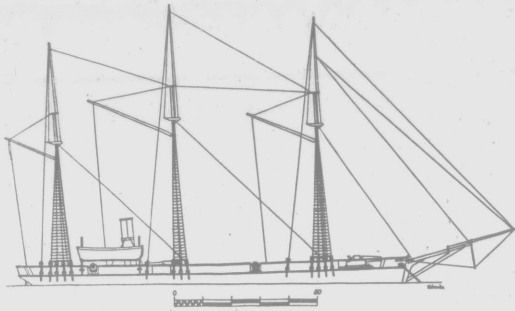
THE CSS CHATTAHOOCHEE — In this illustration by Bob Holcombe, director of the Confederate Naval Museum, the Confederate gunboat appears to be similar to many other schooner-rigged sailing vessels of the Civil War period. Only one stack, aft of the main mast, distinguishes the Chattahoochee as a steam-powered vessel.
