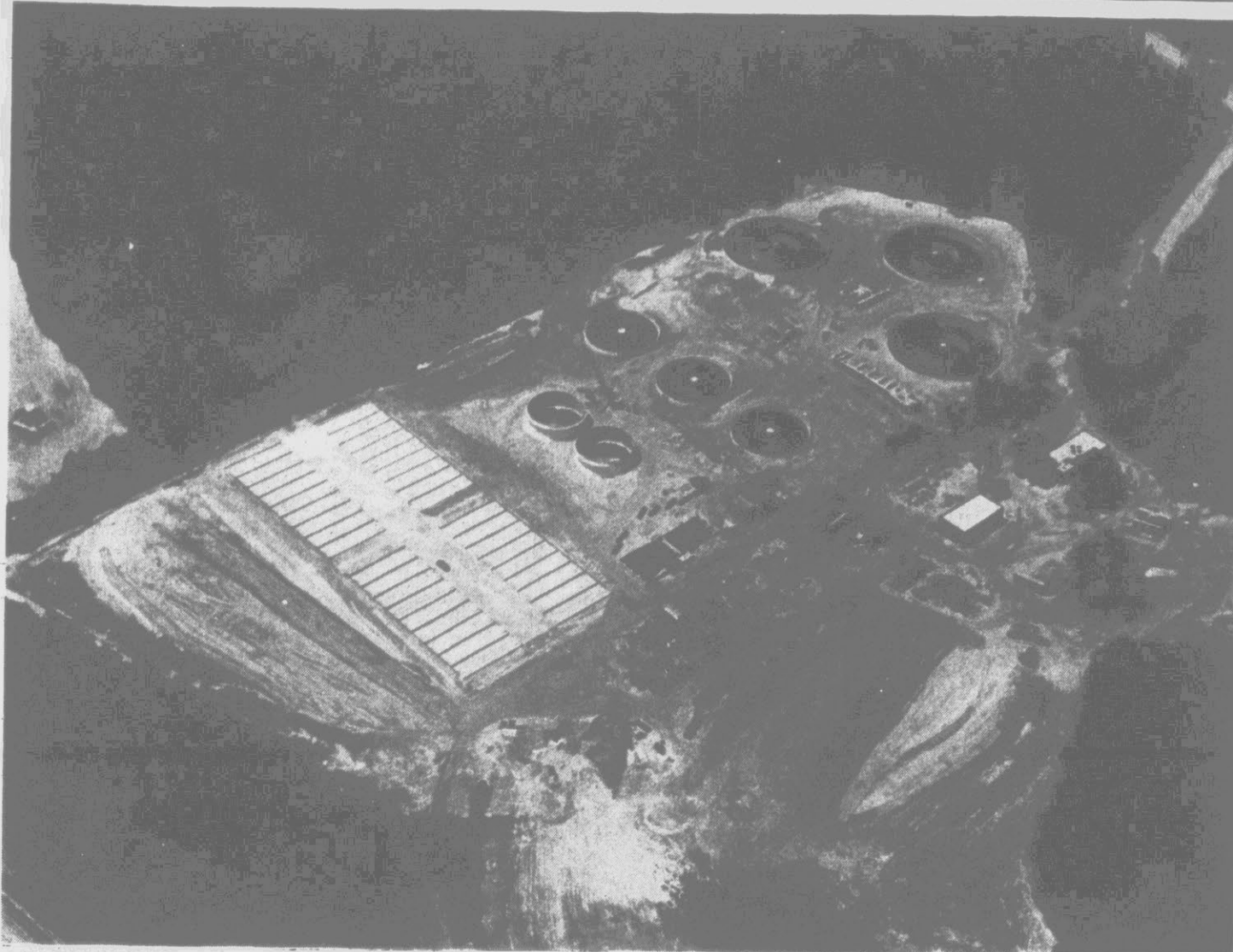
WASTE WATER PLANT ... Construction of the city's new waste water treatment plant is ahead of schedule. The facilities include (from lower left to upper right) sludge drying beds, two sludge holding tanks, three in-line clarifiers where solids are allowed to settle out, and three aeration tanks.
