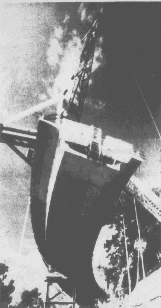
STRUCTURE IN PROGRESS — The Linn Cove Viaduct around Grandfather Mountain, when completed will be 1,243 feet long. The structure is being built for the National Park Service, and its developer claims it includes every kind of alignment geometry used in highway construction. (AP Laserphoto)
