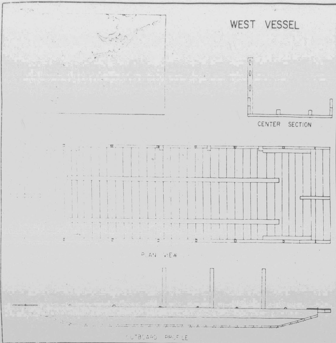
PRELIMINARY DRAWING... This sketch of one of the two submerged ferries, the one designated as the "West" ferry, has been made by Julie Melton and Gordon Watts based on study and survey of the vessels. This sketch, and the one for the
