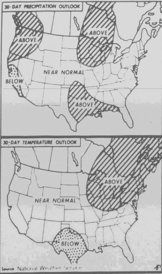
THIRTY-DAY OUTLOOK — Map shows the precipitation ranges and temperature highs and lows for the next thirty days as forecast by the National Weather Service. (AP Laserphoto)
