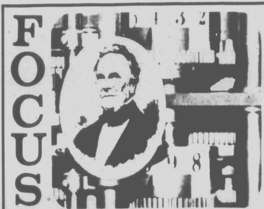
Computer "Roots"
