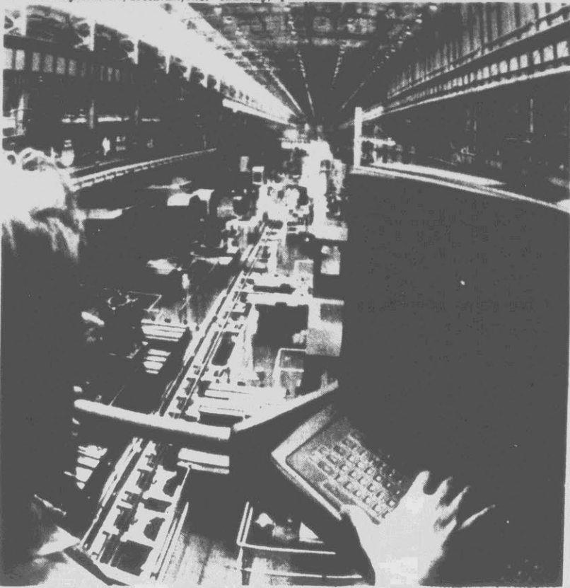
AUTOMATED PLANT — A controller at the General Electric Company Transportation Plant in Erie, Pa., is seated at a computer terminal overlooking the automated Flexible Machine System for traction motor frames for locomotives. The $16 million machine system is the first operational section of what will be a $316 million fully-automated transportation
