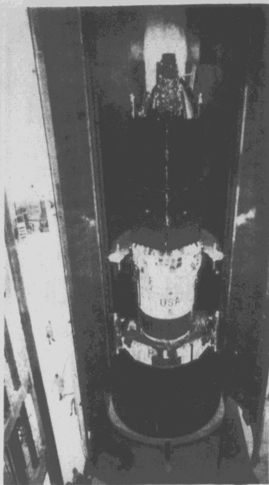
DATA RELAY SATELLITE — Technicians transfer the Tracking and Data Relay Satellite and its upper stage, the primary cargo for the Space Shuttle Six mission, into the transport cannister at Kennedy Space Center. The cargo will be installed in the Space Shuttle Challenger on Jan. 7. The mission is scheduled to begin no earlier than Jan. 27. (AP Laserphoto)
