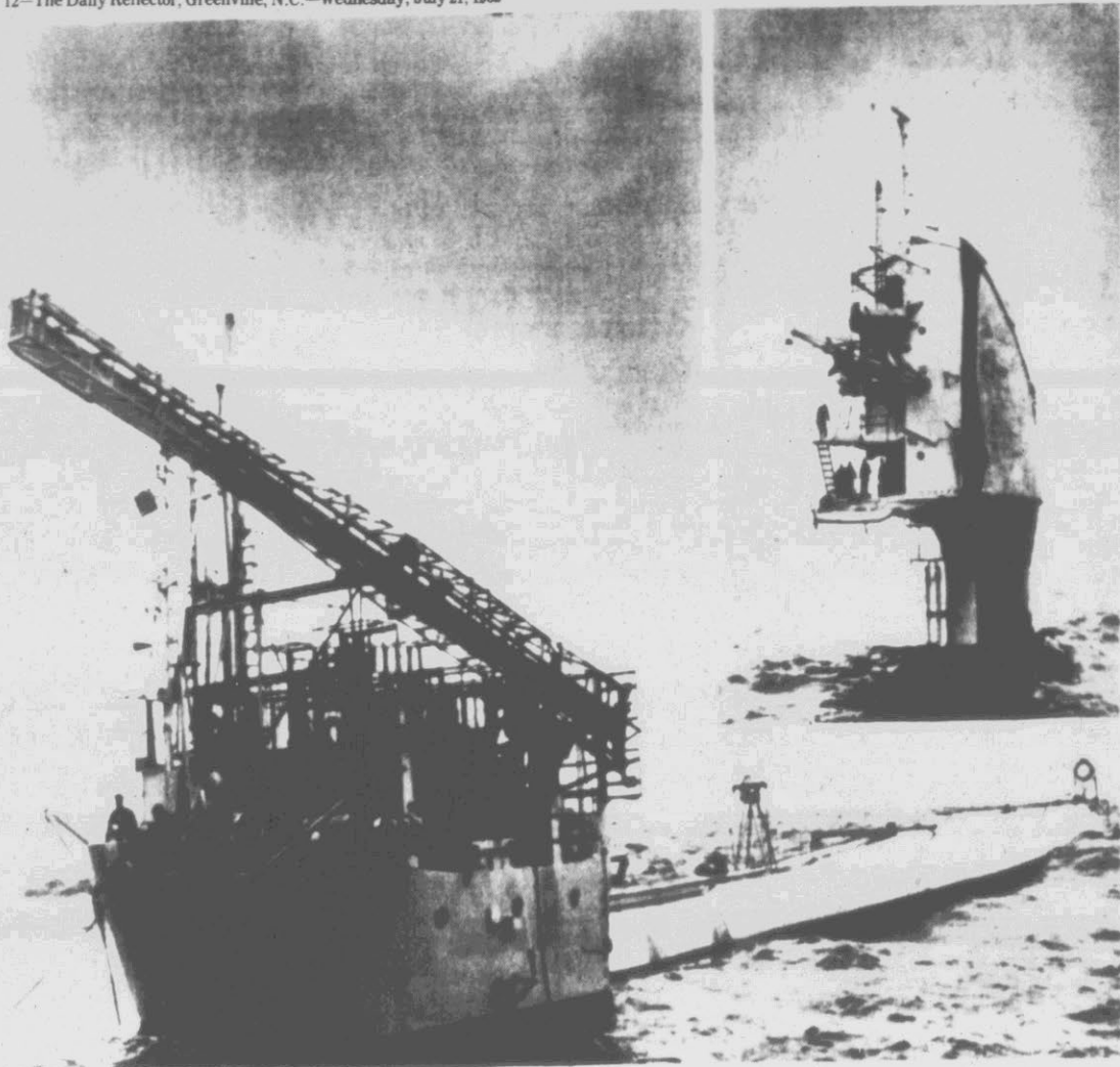
FLIP-FLOP — The Scripps Institution of Oceanography has released these photos to demonstrate how its deep-sea research ship, FLIP, stands on end on command, upper right. The ship, which has now been in use for 20 years, was photographed during a recent visit to the harbor at San Diego. (AP Laserphoto)
