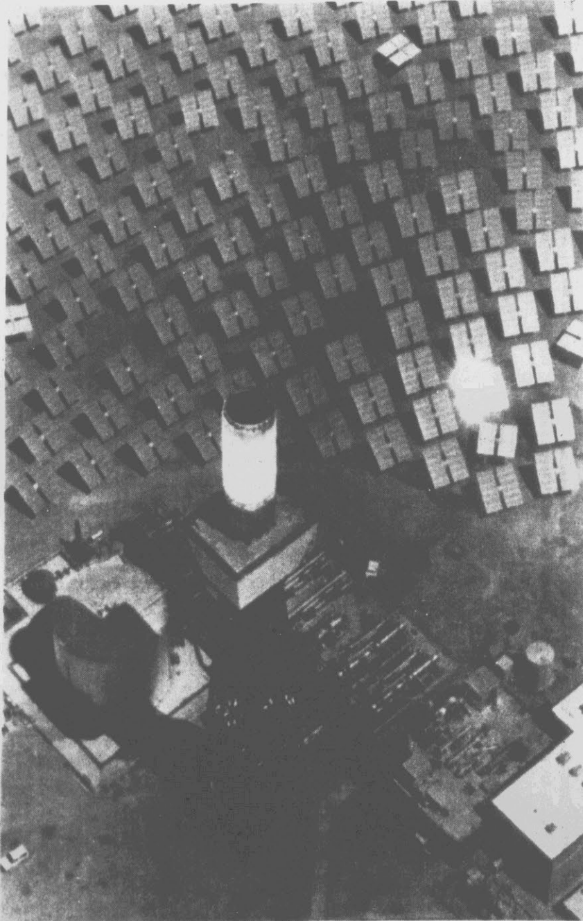
ON THE SUNNY SIDE — A 45-foot boiler atop a 250-foot tower glows brilliantly as sunlight is reflected by the 1,818 racks of mirrors encircling the structure at Solar One, a $141 million pilot plant lauded as the world's largest solar-powered generating plant located southeast of Barstow in the Mojave Desert.
