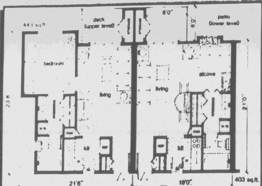
1ST AND 2ND LEVEL FLOOR PLANS
